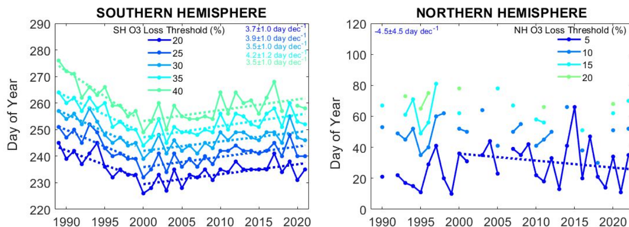
Figure 9. Onset day when 10-day averaged ozone loss reach a particular ozone loss value: 20, 25, 30, 35 and 40% for the SH (left panel) and 5, 10, 15 and 20% for NH (right panel). Robust linear fits before and after 2000 are also shown for the SH (dashed lines).
