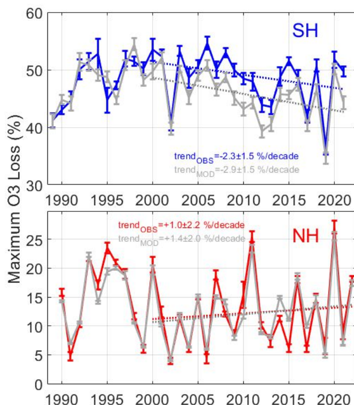
Figure 8. Interannual evolution of the maximum ozone loss obtained using the passive tracer method and the merged OBS dataset (colour lines) and model (gray line) in the SH (top panel) and NH (bottom panel). The estimated robust trends since 2000 were added to the figures with the corresponding colour codes.
