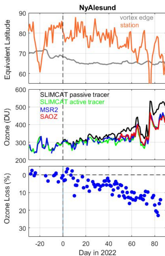
Figure 1. Top panel: evolution of the position of the vortex edge over Ny-Alesund station in equivalent latitude scale at the 475 K isentropic level. Middle panel: evolution of ozone columns at Ny-Alesund from reanalysis MSR2 fields, SAOZ observations and simulated by SLIMCAT. Bottom panel: evolution of ozone loss (in %) at Ny-Alesund derived from OBS merged dataset (see the text) and the SLIMCAT passive tracer.
