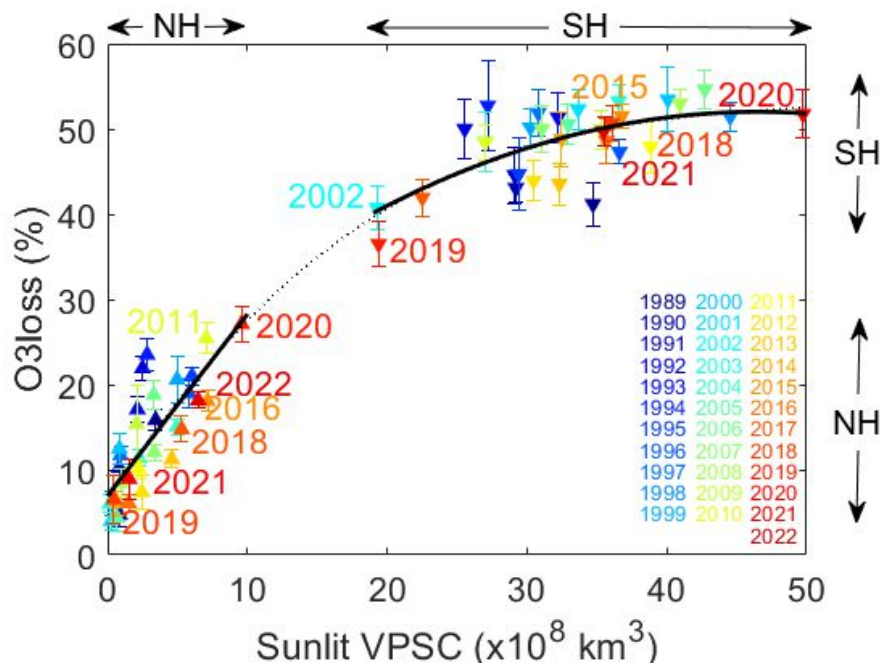
Figure 10. Ozone loss as a function of sunlit volume of polar stratospheric clouds (VPSC) for each winter for the Northern and Southern hemispheres. The 68% interpercentile of ozone losses are also represented (see Sect. 3, Methodology). The colour code represents the years. The linear and parabolic fits are represented for the NH and SH, respectively, (black lines) and the 3 rd -order fit considering years for both hemispheres is represented by the black dotted line.
