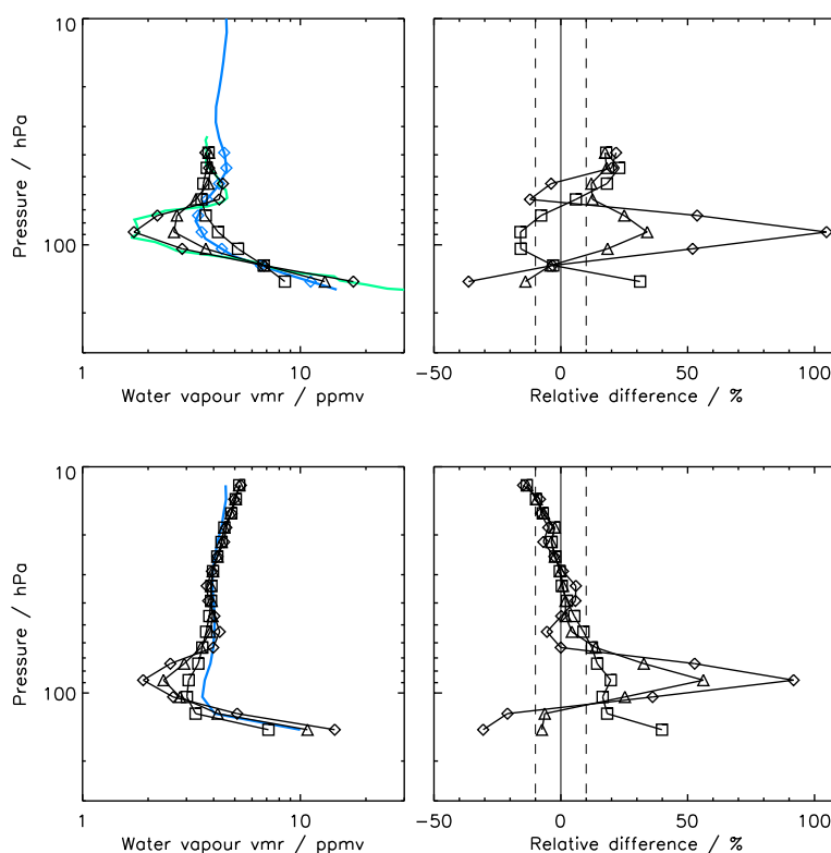
Figure 3. Impact of the different methods for adjustment of the vertical grid and resolution of FP profiles (here: BIK) to those of the satellite data records (here: MIR). Top left: Sample single profiles of satellite (blue) and co-located FP data (green). Black diamonds: FP profile directly interpolated onto the coarse common grid, black triangles: FP profile smoothed with a Gaussian kernel (details see text), black squares: proper averaging kernels and a priori information applied to FP profile. Top right: Corresponding relative differences for the three variants in terms of satellite profile minus FP profile. Bottom left: Averaged profiles for coincident MIR (blue) and FP data at BIK (black, symbols as for data shown in top row plot frames). Bottom right: Corresponding relative differences for the three variants in terms of satellite profile minus FP profile, divided by FP profile.
