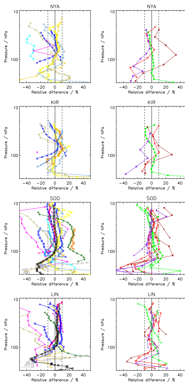
Figure A4. Mean relative differences between the FP stations NYA, KIR, SOD, LIN and coincident SAT records (left: data records except MIPAS; right: only MIPAS data records). Color coding of the SAT data according to Fig. 2.
