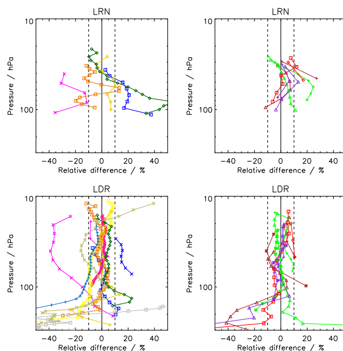
Figure A10. Same as Fig. A4 but for LRN and LDR.
