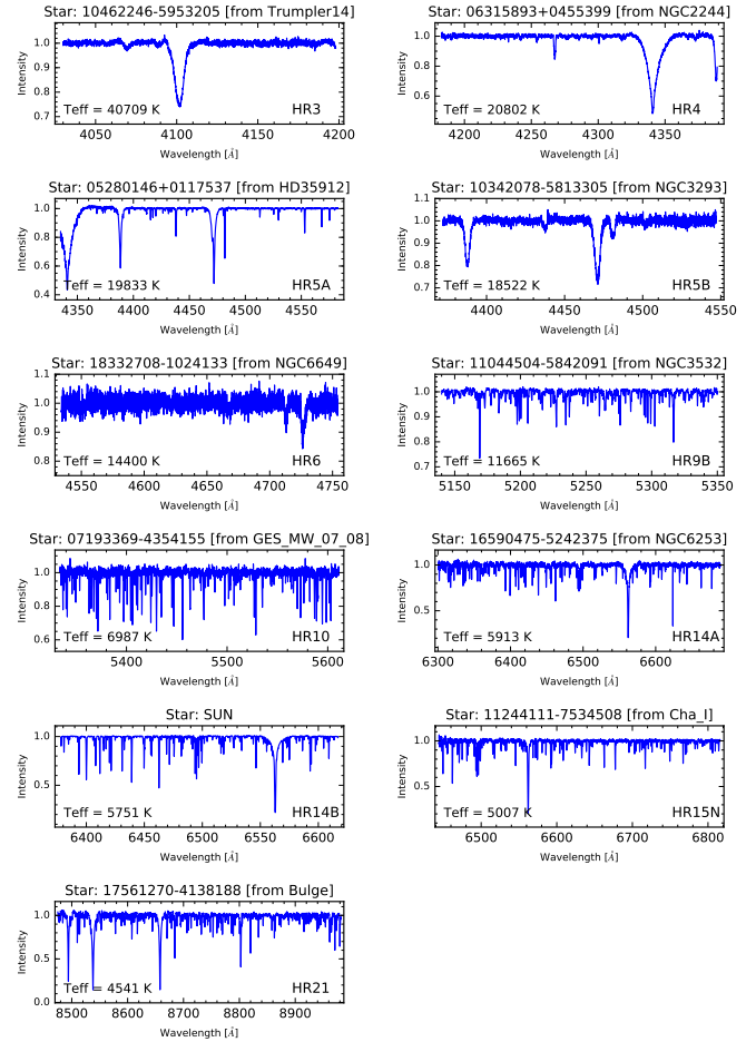
Fig. 10. Example spectra from several GIRAFFE setups.
