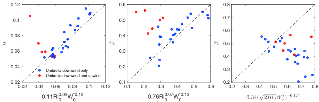
Figure 5. Estimated value of \alpha or \beta compared to functions of the form C_1 R_i^r W_0^{*w_1} . (left and middle) Fit parameters C_1 , r_1 , and w_1 are estimated using a multilinear regression between \alpha or \beta , and R_i and W_0^* , on a log scale. Only plumes for which the umbrella spreads only downwind (blue) are used to perform multilinear regressions. (right) The estimated values of \beta as a function of the parameterization used in model 3. Dashed lines show the 1:1 ratio. The estimates of \alpha and \beta are subject to large uncertainties which are not shown for clarity.
