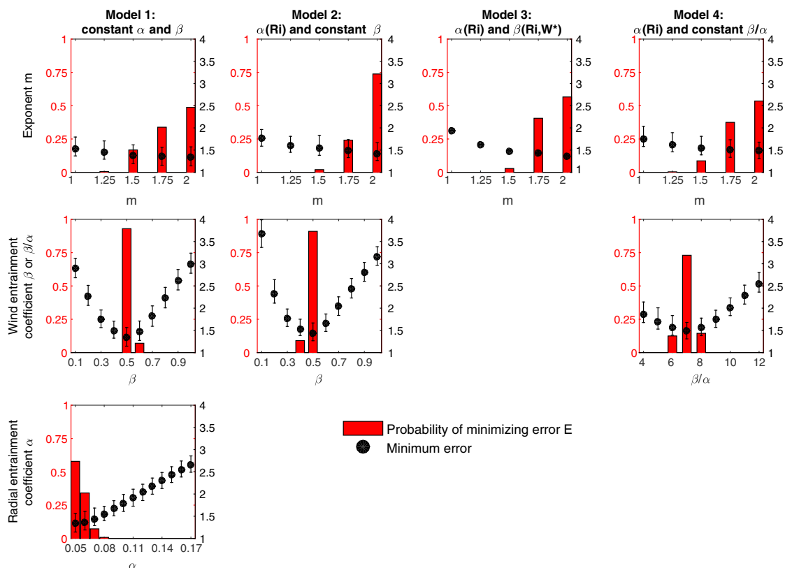
Figure 2. Values of plume model parameters minimizing the error on centerline trajectory (equation (12)). Each column of plots shows results related to one entrainment model, while each row of plots shows results related to one type of model parameter. On each plot, red bars (left red axis) show the distribution (across all Monte Carlo simulations) of the parameter values for which the error E on centerline trajectory is minimized. Black dots (right black axis) show the minimum error on centerline trajectory for a fixed value of the model parameter considered. Dots show the mean error and error bars are the 95% confidence interval.
