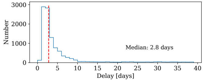
Fig. 4. Histogram of the delay (in days) between the Gaia observation and the publication of an alert. The long tail is the result of allowing the two FOVs that we require the alert to be seen in, to be separated by up to 40 days. Twelve per cent of the alerts have a publication delay longer than 10 days. The median delay is 2.8 days and is indicated by a dashed vertical line.
