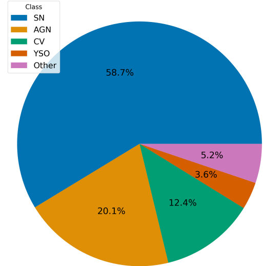
Fig. 11. Distribution of the most common classifications for alerts from GSA. As discussed in the text, there is strong bias in the rate of follow-up and classification in favour of events which look like supernovae or other extragalactic transients.
