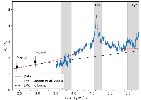
Fig. 2. Derived extinction curve from the dust in the absorber. The contribution from the quasar dust has been removed to highlight the 2175 \text{\AA} dust bump from the absorber. The dashed line shows the LMC extinction curve by Gordon et al. (2003) and the dotted line shows the same extinction curve but with no bump. The position of emission lines is indicated by the shaded bands. Narrow peaks are caused by differences between the intrinsic quasar spectrum and the template used in the analysis.
