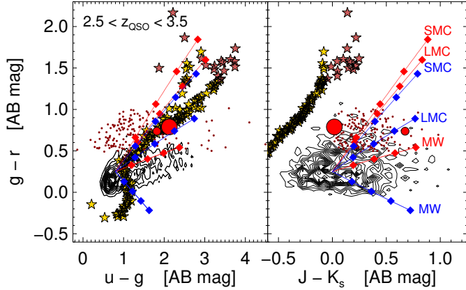
Fig. 4. Colour-colour distributions of the SDSS/BOSS-DR12 quasar sample in the redshift range, 2.5 < z < 3.5 (black contours). The reddening has moved eHAQ0111+0641 (shown with a large red circle) away from the quasar locus onto the stellar track indicated with yellow (normal stars) and red (M-dwarfs and later) stars. The small red circle shows the position of HAQ2225+0527 discussed in Krogager et al. (2016a), which also falls on the stellar track in the SDSS colours. In the near-IR the object is well separated from the stellar track. The dark red points show the distribution of 150 HAQs from Krogager et al. (2015). Also plotted are the reddening vectors for a z = 3 quasar reddened by SMC, LMC, and MW extinction curves from Pei (1992) at foreground redshifts of 2.0 (blue lines) and 2.5 (red lines). The diamonds along the lines show the points corresponding to A_V s of 0.5, 1.0, 1.5, and 2.0.
