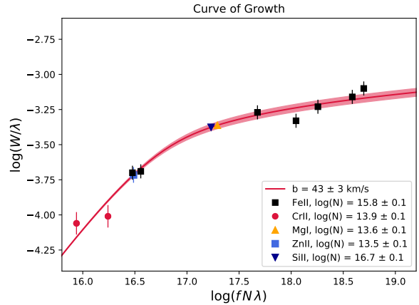
Fig. 3. Curve of growth (COG) for Fe II lines from the z = 2.027 DLA. The other species are assumed to follow the same COG and are plotted for comparison. The red shaded area indicates the 1\sigma uncertainty on the b parameter.
