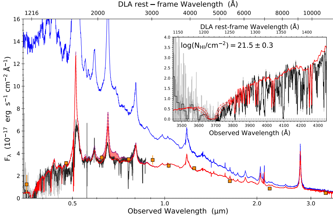
Fig. 1. GTC spectra shown together with the photometry from SDSS, UKIDSS, and WISE in the u, g, r, i, z, Y, JH, Ks, and W_1 bands (Warren et al. 2007; Wright et al. 2010; Eisenstein et al. 2011). We also overplot a composite quasar spectrum and a reddened composite as described in the text. The shaded area shows the effect of the 2175- \text{\AA} extinction bump from dust in the z = 2.027 DLA galaxy. In the inset we plot a zoom on the blue part of the spectrum where we show the 2500U spectrum covering the region around the hydrogen Ly \alpha line of the z = 2.027 absorber. Overplotted is the DLA fit assuming a column density of 10^{21.5 \pm 0.3} \text{ cm}^{-2} ; the \pm 1\sigma curves are shown with dashed lines.
