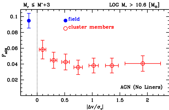
Figure 7. Variation of AGN fraction as a function of normalized relative velocities ( \Delta v / \sigma_v ) displayed as red open circles. The corresponding estimate for the field is indicated by the blue filled circle. The error bars indicate the 1\sigma standard error on the biweight location estimate. [A colour version of this figure is available in the online version.]
