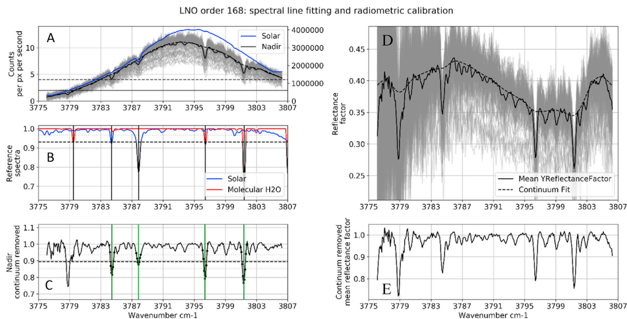
Fig. 15. Reflectance factor conversion steps for a single LNO nadir observation. [A]: The spectra are normalised to raw counts per pixel per second. Those with the highest SNR are averaged together to make a mean spectrum (solid black line) and a synthetic solar spectrum is created for same the instrument temperature (blue line). The nadir continuum is fit (dotted black line) and divided to produce a nadir flattened spectrum (C, black line). [B]: simulated reference molecular (red) and solar spectra (blue) are analysed to find the wavenumbers of possible absorption lines (black vertical lines). [C]: Observable absorption lines outside the noise level are found in the mean nadir flattened spectrum (green vertical lines). The nadir spectra are shifted so that the detected absorption lines match the simulated spectra. [D]: the shift-corrected nadir spectra are divided by the solar spectra and variables in Equation (1) to convert to reflectance factor (grey lines). [E]: an example of the mean reflectance factor spectrum once the continuum has been removed. The main solar line at 3788 cm -1 has been suppressed by the conversion to reflectance factor.
