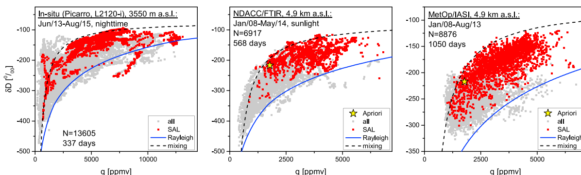
Figure 8. Example of \{q, \delta D\} pair distributions observed in the North Atlantic subtropical free troposphere during several years and by three different techniques, (left) in situ, (middle) ground-based remote sensing (MUSICA NDACC/FTIR), and (right) space-based remote sensing (MUSICA MetOp/IASI). Grey dots represent all observations, red dots observations during Saharan Air Layer (SAL) events, and the yellow star is the a priori \{q, \delta D\} pair used for all remote sensing retrievals. In addition, the plots show two simulated curves: (1) A Rayleigh curve (blue line) for initialization with T = 25^\circ\text{C} , \text{RH} = 80\% , and \delta D = -80\text{‰} . (2) A mixing curve (black dashed line) for mixing between \{25,000 \text{ ppmv}, -80\text{‰}\} and \{500 \text{ ppmv}, -500\text{‰}\} . For more details please refer to González et al. [2016].
