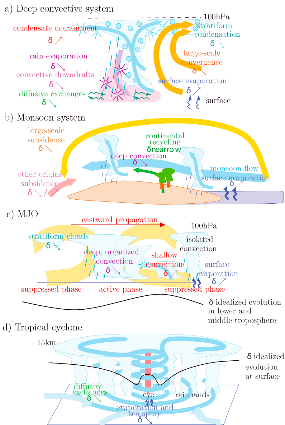
Figure 17. Effect of deep convection and several tropical weather and climate features on the isotopic composition of water vapor: (a) deep convection, (b) monsoon, (c) Madden-Julian Oscillation, and (d) tropical cyclone.
