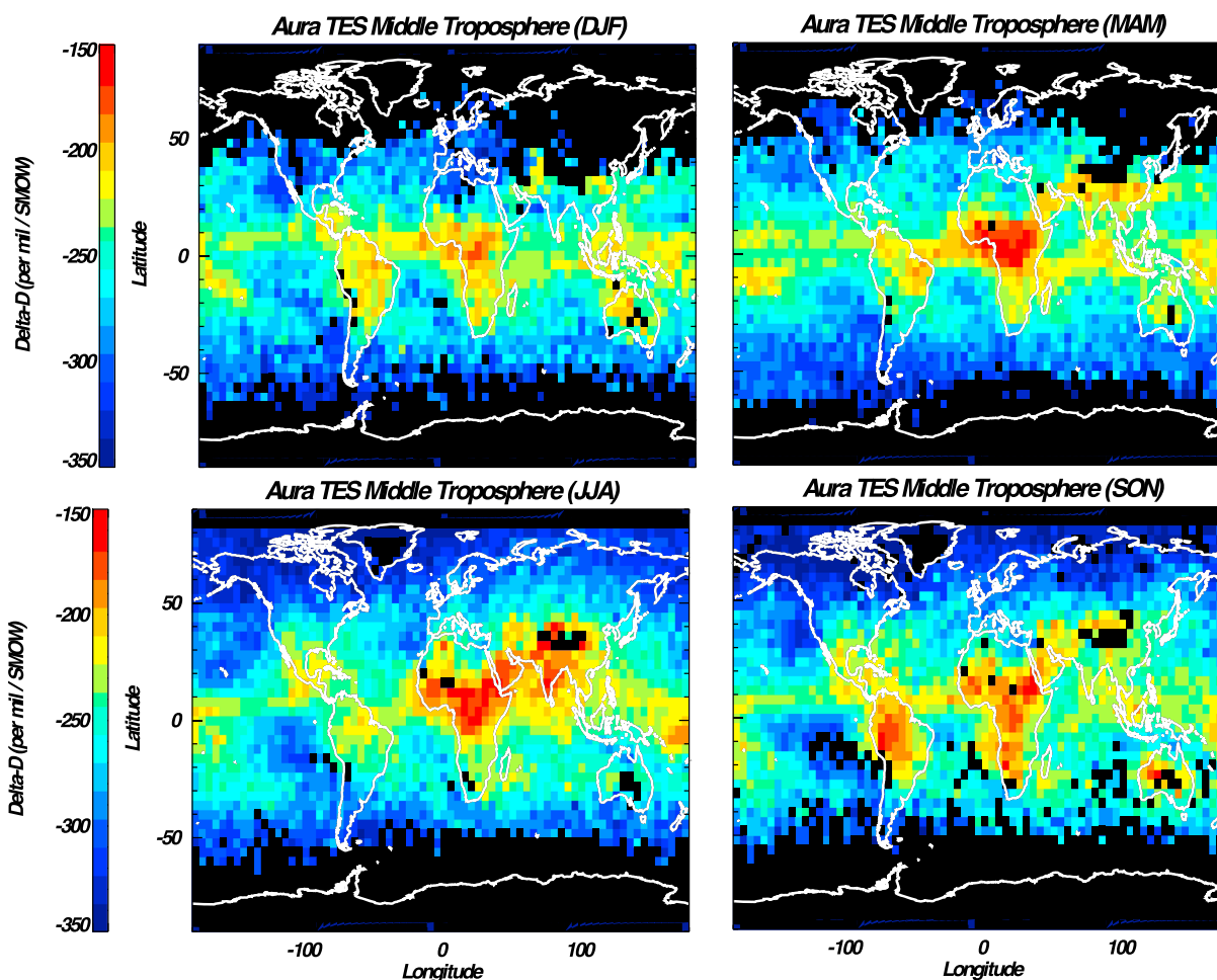
Figure 12. Seasonal average \delta D for the middle troposphere defined as the layer between 300 hPa and the top of the “lower troposphere” shown in Figure 11.
