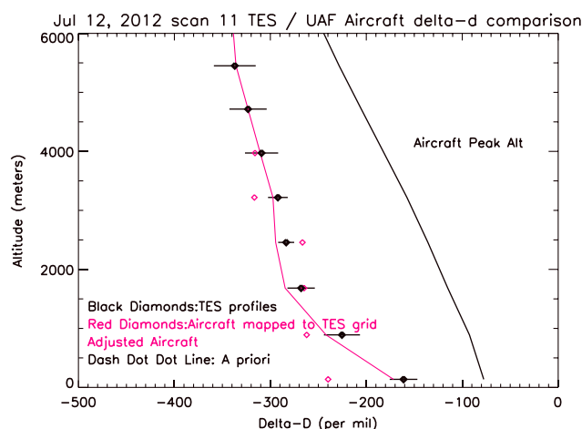
Figure 6. Comparison of a TES retrieval to aircraft measurements. The dashed line is the a priori used for the TES retrieval. The red diamonds are the raw aircraft measurements, mapped to the TES retrieval grid. The solid red line is the aircraft measurement after passing through the TES instrument operator. The black diamonds show the TES HDO/H 2 O profile (in units of per mil relative to SMOW).
