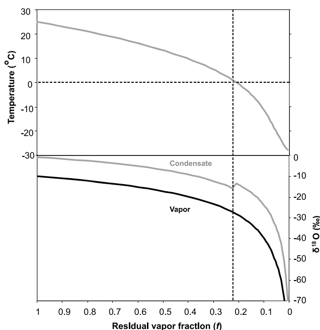
Figure 2. Isotopic composition of a precipitating air mass with vapor depleting according to the Rayleigh model with an initial vapor composition of \delta^{18}\text{O} = -10\text{‰} at T = 25^\circ\text{C} , following Clark and Fritz [1997]. The dashed lines indicate the transition from rain to snow.
