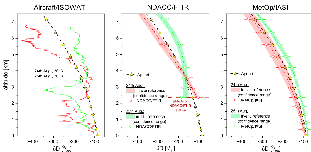
Figure 7. Example of vertical distribution of tropospheric \delta D measured on two consecutive days in coincidence by three different techniques. Day 24 August can be identified by red and day 25 August by green color. Dashed black line with yellow stars is the a priori used by the remote sensing retrievals. (left) In situ measurements by ISOWAT from aircraft; (middle) Circles and error bars represent MUSICA NDACC/FTIR remote sensing observations and their uncertainty, colored dashed line and shaded area represent the in situ references and their confidence range after considering the vertical resolution and sensitivity of the FTIR retrievals; (right) same as Figure 7 (middle) but for the MUSICA MetOp/IASI remote sensing observations. For more details please refer to Dyroff et al. [2015] and Schneider et al. [2016].
