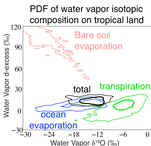
Figure 16. Probability density function of the isotopic composition ( \delta^{18}\text{O} and d -excess) of water vapor at the lowest model level for all tropical land locations and for all days in 2006, for total vapor (black), vapor originating from ocean evaporation (blue), vapor originating from land surface transpiration (green), and vapor originating from bare soil evaporation (pink). These probability density functions are calculated from a model simulation equipped with the water-tagging technique [Risi et al., 2013].
