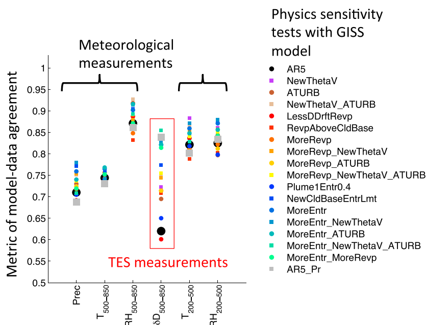
Figure 15. GISS GCM agreement across a small ensemble of 18 perturbed physics experiments for different observation types across the tropics for 2005–2011 [Field et al. , 2014]. The metric of model data agreement is the spatial pattern correlation between model and observations in the annual mean. The greater spread in agreement for \delta D suggests that these measurements have unique potential beyond conventional observations for model evaluation.
