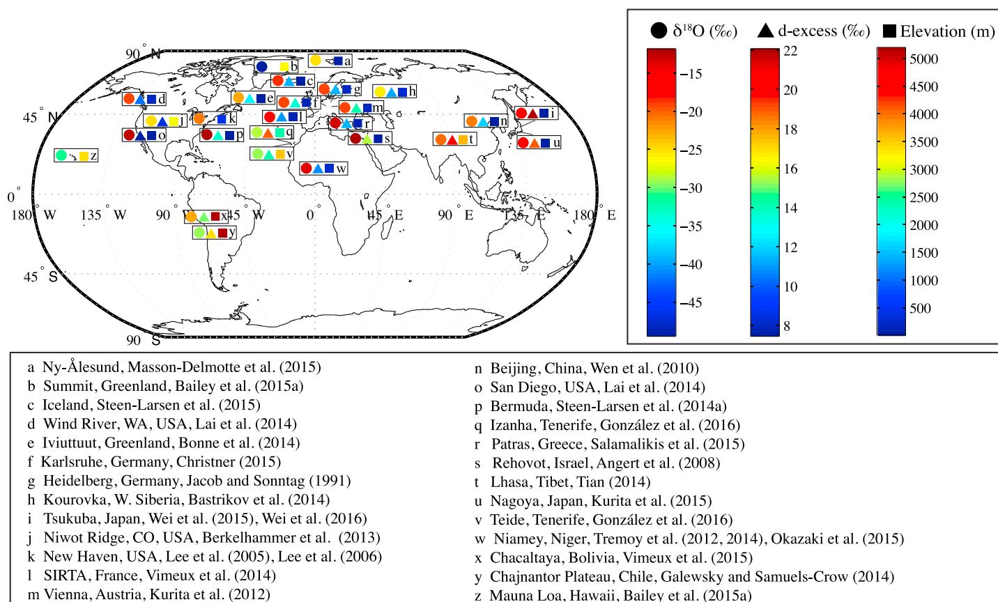
Figure 10. Mean annual in situ water vapor \delta^{18}\text{O} and d -excess (where data are available) from stations with at least one full year of measurements together with elevation of measurement station. The \delta^{18}\text{O} value is given by the color scale of the filled circle (spanning -11\text{‰} to -50\text{‰} ), the d -excess is given by the color scale of the filled triangle (spanning 8\text{‰} to 22\text{‰} ), and the elevation is given by the color scale of the filled square (spanning sea level to 5200\text{ m} ).
