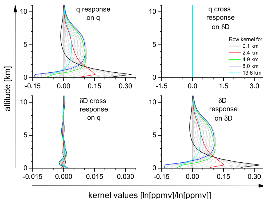
Figure 5. Example of row entries of the Karlsruhe MUSICA NDACC/FTIR averaging kernels in the \{q, \delta D\} proxy basis system and after a posteriori correction. Please note that the (top left) q proxy kernels and the (bottom right) \delta D proxy kernels are almost identical. The different scales on the x axis consider the different magnitudes of \ln[q] and \delta D variations. For more details please refer to Schneider et al. [2012] and Barthlott et al. [2016] .
