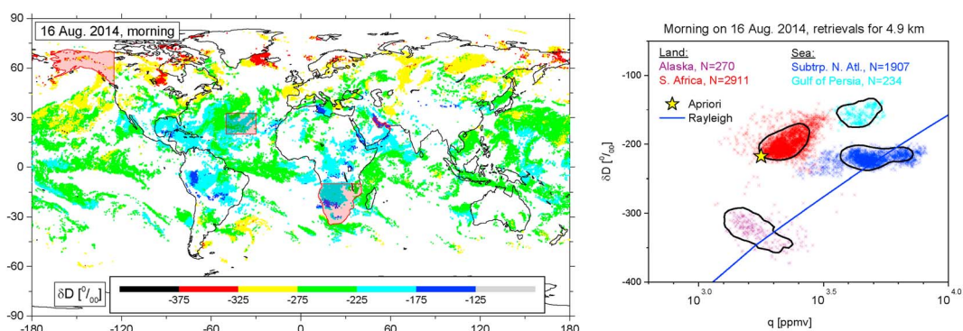
Figure 13. Example of MUSICA MetOp/IASI \{q, \delta D\} pair observations in the middle troposphere during a single morning overpass (at about 10 local time). (left) Daily \delta D morning overpass map (similar coverage is achieved for an evening overpass at about 22 local time). (right) Distinct \{q, \delta D\} pair distributions observed in the four different regions as marked by reddish color in the left map. The black lines envelop the \{q, \delta D\} area with the highest data point density and with 66% of all data points. N gives the number of individual observations in each region. The blue line is an example Rayleigh curve (same as in Figure 8). For more details please refer to Schneider et al. [2016].
