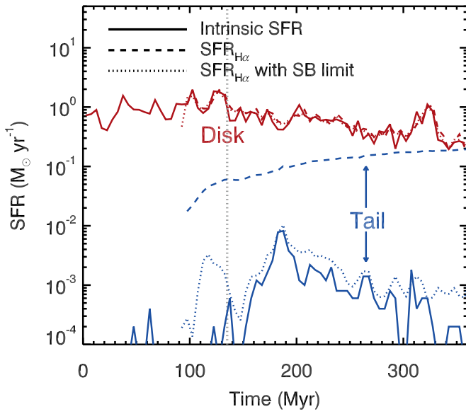
Figure 12. Evolution of the intrinsic SFR (solid) and the SFR estimated from the total unobscured H\alpha luminosity ( SFR_{H\alpha} ; dashed and dotted). The red and blue colors indicate the SFRs in the disk and tail, respectively. We present SFR_{H\alpha} with (dotted) and without (dashed) an SB limit of 6 \times 10^{38} \text{ erg s}^{-1} \text{ kpc}^{-2} . We display the SFR_{H\alpha} lines only at t > 100 \text{ Myr} . The vertical dotted line marks the epoch at which the wind front reaches the galaxy. SFR_{H\alpha} closely traces the intrinsic SFR in the disk, while the majority of the H\alpha SB (dashed) in the tail originates from processes other than star formation. However, the intrinsic SFR in the tail is reasonably recovered by considering H\alpha bright regions (dotted).
