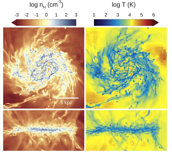
Figure 2. Projected views of the gaseous disk of the simulated galaxy. The panels display the face-on (top) and edge-on (bottom) views of density-weighted distribution of the hydrogen number density (left) and temperature (right) from the NoWind_rich galaxy at t = 135 Myr, i.e., the moment at which the ICM wind starts influencing the galaxy.
