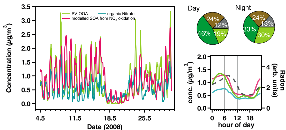
Figure 2. Time series of the mass concentrations of measured organic nitrate and SV-OOA and modeled SOA from \text{NO}_3 oxidation at Cabauw during May 2008. Inserts show the average diurnal including also Radon concentration (grey dashed line, right axis) as boundary layer dilution tracer and day and night pie charts of the relative contribution of individual organic PMF factors.
