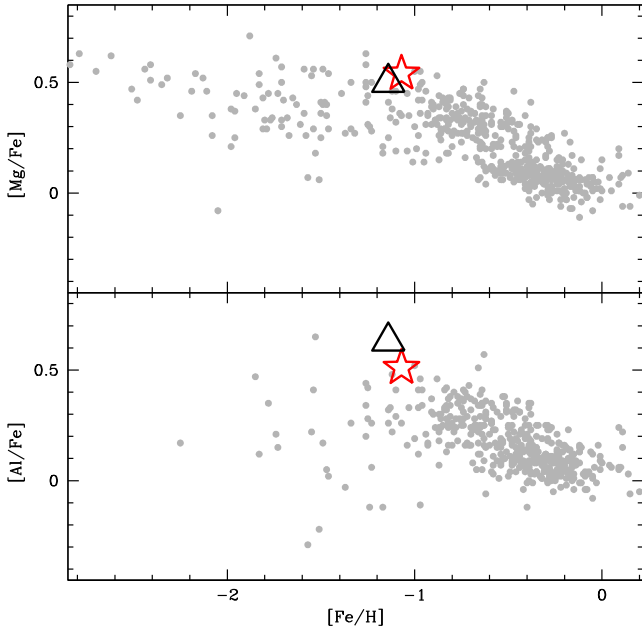
Figure 3. Upper panel: [\text{Mg}/\text{Fe}] versus [\text{Fe}/\text{H}] trends for NGC 6362 (red star) and M 4 (black triangle), compared to a sample of field stars (grey dots). Lower panel: same comparison for [\text{Al}/\text{Fe}] .
