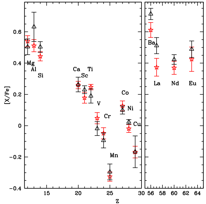
Figure 7. Comparison among the elemental abundances measured for NGC 6362 (red stars) and M 4 (black triangles).
