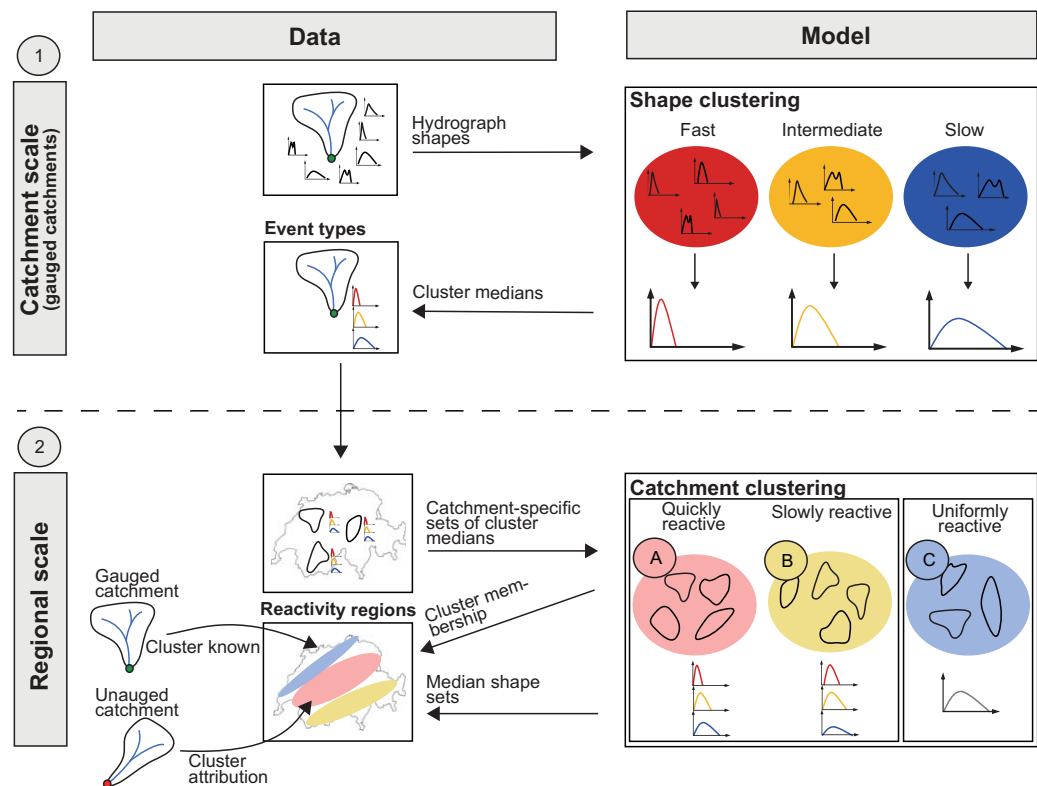
Figure 3. Illustration of the clustering framework. The data input and output for the models are indicated for the two different parts: (1) hydrograph shape clustering, (2) catchment clustering. Hydrograph shape clustering is done on the catchment scale and catchment clustering on the regional scale.
