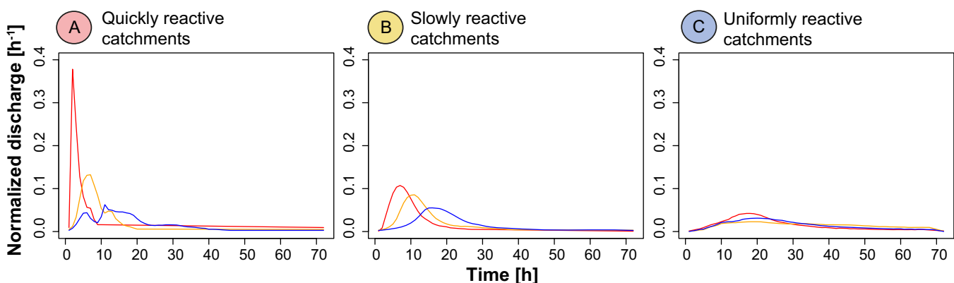
Figure 6. Fast, intermediate, and slow median hydrograph shapes for three catchments: (a) Alp-Einsiedeln (quickly reactive region), (b) Arbonne-Avenches (slowly reactive region), and (c) Birs-Münchenstein (uniformly reactive region).
