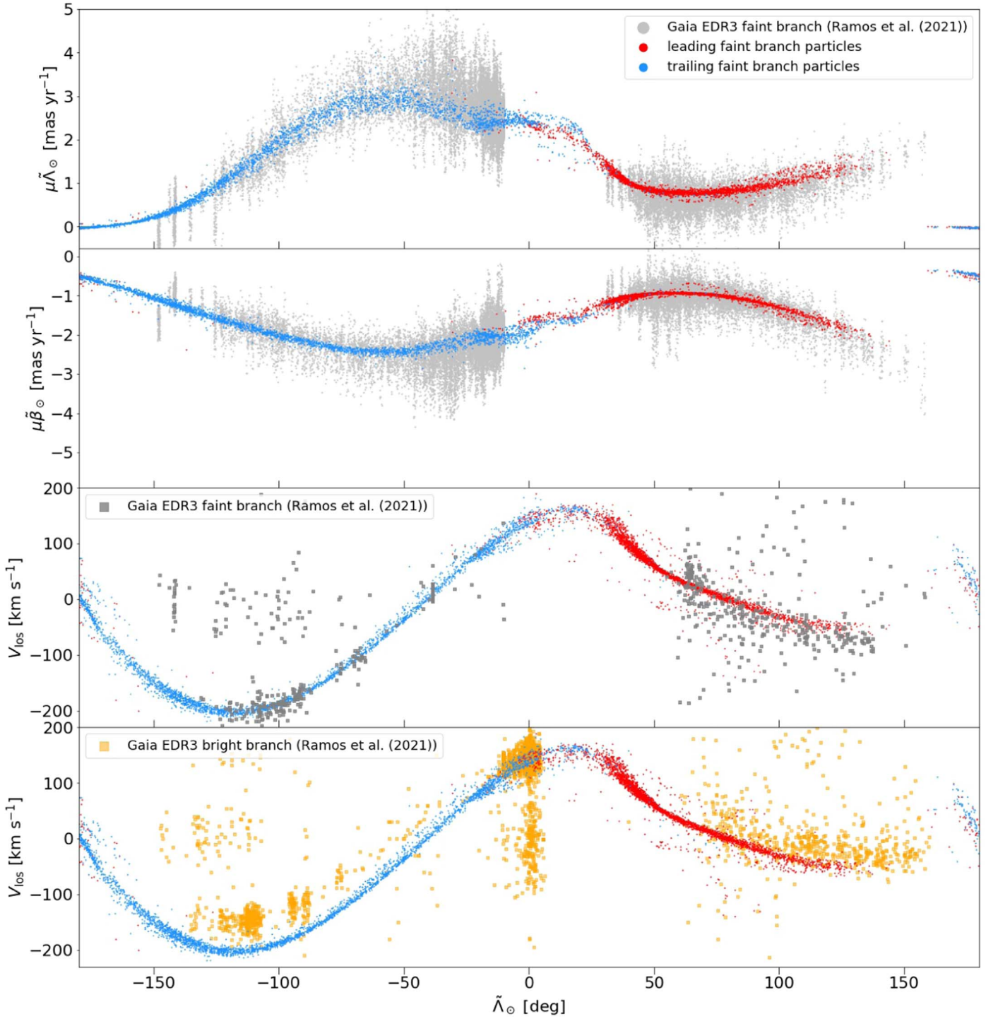
Figure 5. Comparison of the faint branch (probability \geq 80\% ) from the Gaia EDR3 Sgr sample of Ramos et al. (2021, gray) with the faint branch selection in our N -body model including self-gravity (red for the leading arm, blue for the trailing arm). From top to bottom: proper motions in \tilde{l}_0 , in \tilde{b}_0 , and line-of-sight velocities (heliocentric reference frame). For comparison, the bottom panel shows bright branch members (probability \geq 80\% , yellow).
