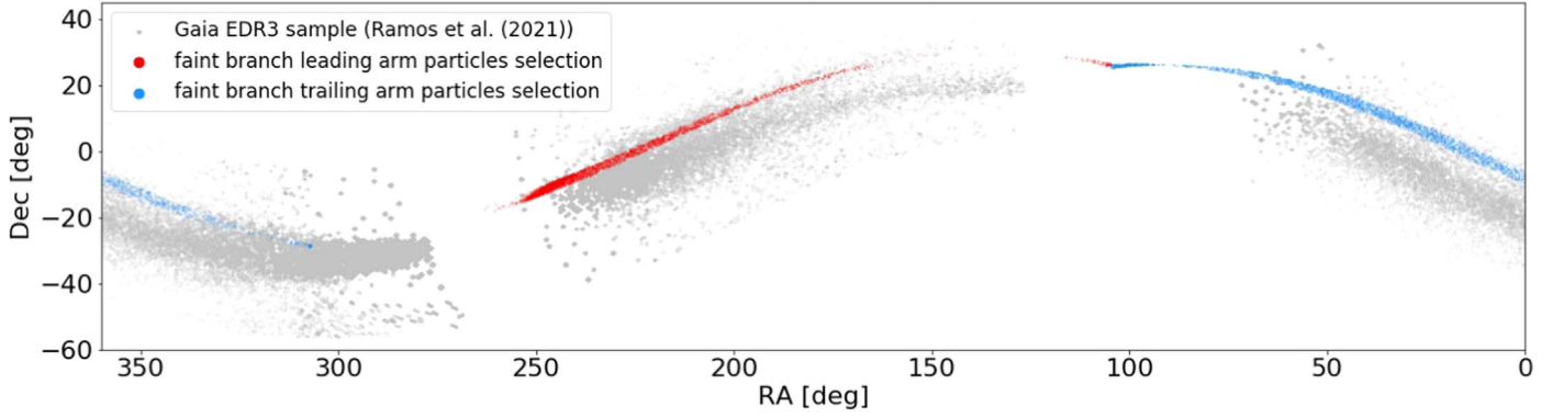
Figure 1. The Gaia EDR3 Sgr sample from Ramos et al. (2021) in the background (gray), with our selection of faint branch test particles from our simulations from Section 3.1.1 overplotted (red for leading arm, blue for trailing arm). The remnant of the progenitor lies in the 275^\circ \leq \text{R. A.} \leq 300^\circ region.
