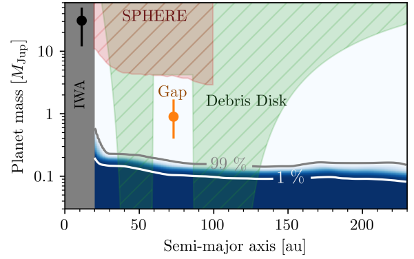
Fig. 6. JWST MIRI 15 \mu\text{m} detection probability as a function of planet mass and semimajor axis for a 1 h integration, taking into account the system's inclination, age uncertainty, and probability of reaching a 5\sigma level. The contours show the 99 and 1% probabilities. The orange error bar shows the predicted planet carving the gap. The red and green hatched regions are excluded since no planets were detected with SPHERE (red) and a planet in that region would disrupt the disk or push their edges away from where they are observed with ALMA (green). The gray region represents the inner working angle (IWA) of JWST in this mode.
