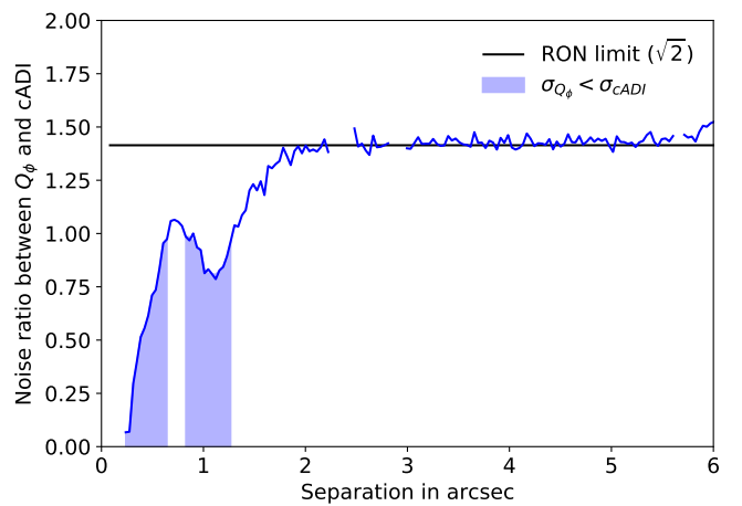
Fig. 3. Ratio between the azimuthal noise profile in the Q_\phi image and in the cADI-reduced image; both images come from the same observations. The asymptotic value (black line) of \sqrt{2} = 1.4 in the readout-noise (RON) limited region comes from the fact that only half the frames are used to obtain the Stokes Q image (respectively Stokes U ) when the HWP has a position angle of 0^\circ and 45^\circ (respectively 22.5^\circ and 67.5^\circ ). The sensitivity is higher in the Q_\phi image compared to the cADI image in the blue-shaded area below 1.28'' .
