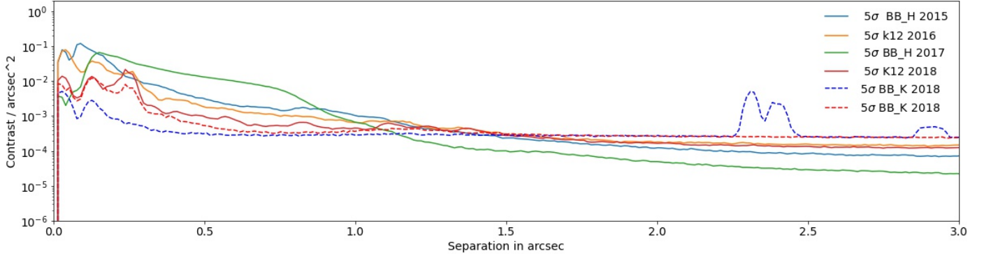
Fig. 2. Five \sigma contrast expressed per arcsec squared for the four CI-DBI data sets (solid lines), as well as for the DPI data set (dashed lines). Two epochs combined, but we distinguished the polarimetric reduction from the ADI reduction.
