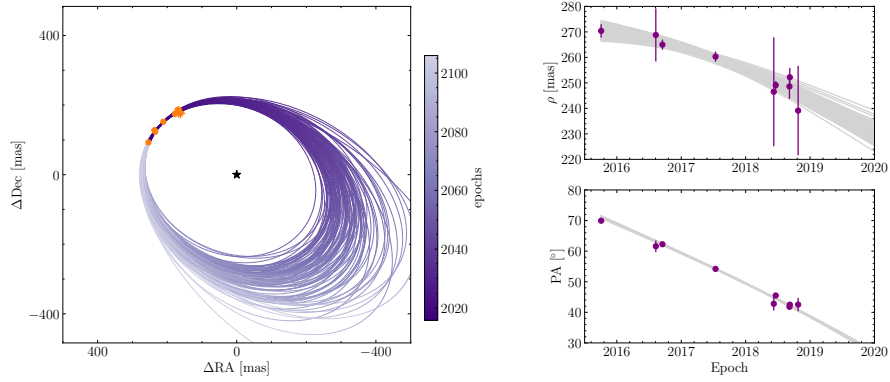
Fig. B.1. Possible orbits for HD 206893 B ( left ) using the same methodology as Marino et al. (2020) and adding the astrometric points from the polarimetric data. The data points are shown in orange, and the respective separations and parallactic angles are shown on the right .
