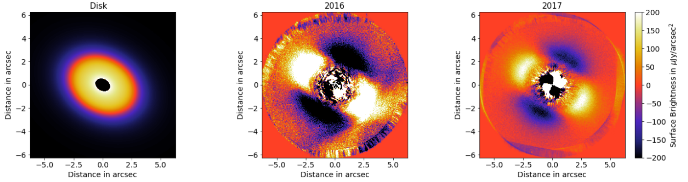
Fig. 4. Simulation of the disk injected in the 2016 and 2017 data sets. The synthetic disk as described by Marino et al. (2020) is shown on the left . The images processed with cADI including the injected disk are shown in the center and on the right for the 2016 and 2017 data sets, respectively. This illustration corresponds to a disk with an albedo equal to 0.9 in the K band (2016) and an albedo equal to 0.7 in the H band (2017).
