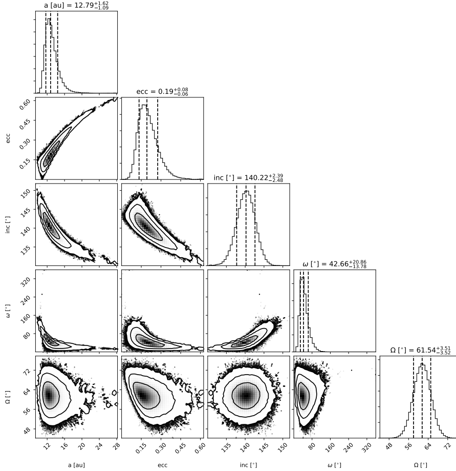
Fig. B.2. Posterior distribution of the semimajor axis, eccentricity, inclination, argument of pericenter, and longitude of ascending node. The vertical dashed lines represent the 16th, 50th, and 84th percentiles, and the contours the 68, 95, and 99.7% confidence regions. This plot was generated following the same procedure used by Marino et al. (2020) .
