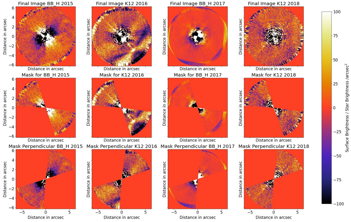
Fig. A.1. Reduced images ( top row ), mask created to segment the area of interest where the disk would be ( middle row ), and its perpendicular to make the comparison between them ( bottom row ).
