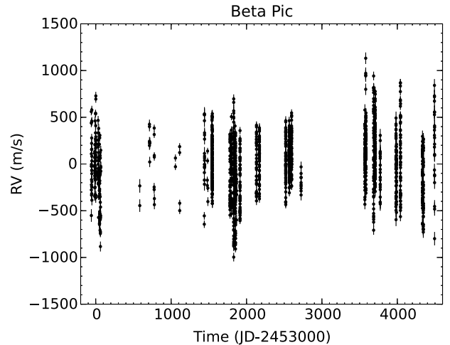
Fig. 1. Top: HARPS RV time-series of \beta Pictoris.
