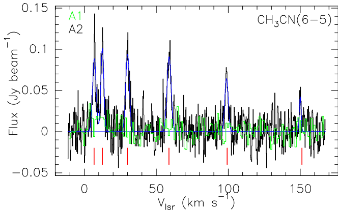
Fig. 3. CH 3 CN ( J = 6-5 ), K = 0-5 spectrum observed in IRAS 4A with PdBI, corresponding to the continuum peak coordinates of A1 (green) and A2 (black). The spectrum of A1 was smoothed to a channel width of 1 km s -1 . The Gaussian fits to the lines detected in A2 are depicted in blue (see Table 2). The positions of the different K transitions, from K = 0 (left) to K = 5 (right), are indicated in red.
