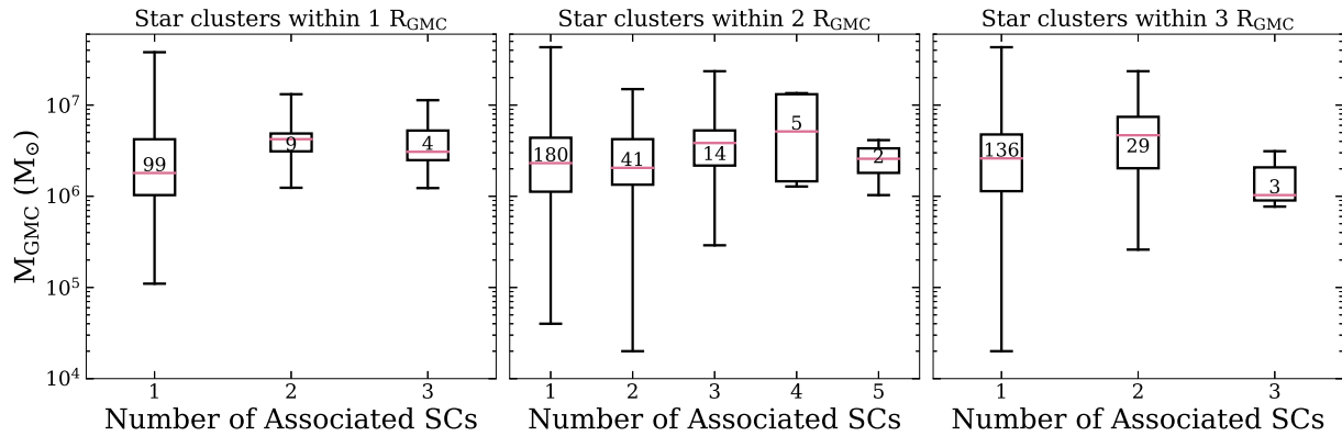
Figure 9. Box plots of the GMC masses versus the number of associated star clusters. The numbers listed in the middle of each box show the total number of each GMC for a given number of associated star clusters and the pink line shows the median of the GMC masses. The box encloses 50 percent of the distribution (the first and third quartiles) and the whiskers extend to the minimum and maximum. The left-hand panel shows the GMC mass distribution for the 118 GMCs with 129 star clusters within one radius of the cloud, the middle panel shows the mass distribution for the 242 GMCs with 334 star clusters between one and two radii of each cloud, and the right-hand panel shows the mass distribution for the 168 clouds with 203 star clusters between two and three radii.
