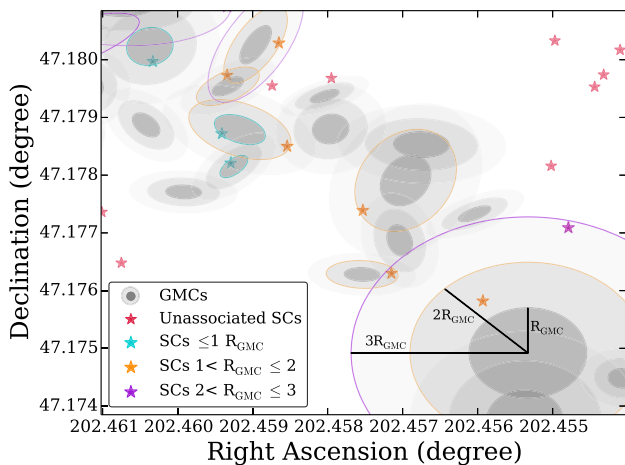
Figure 7. Associated star clusters located inside 1R_{\text{GMC}} (turquoise), 1\text{--}2R_{\text{GMC}} (orange), and 2\text{--}3R_{\text{GMC}} (purple), while unassociated star clusters are shown in pink. We consider star clusters to be associated with a GMC if they lie within the footprint of the molecular cloud. GMCs that have a corresponding cluster are outlined in the same colour as the radial location of the cluster.
