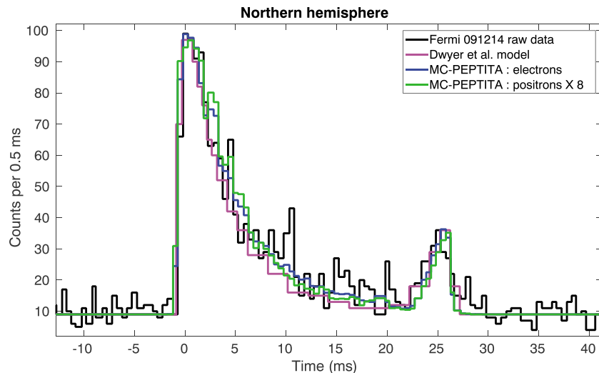
Figure 1. Time histogram of the Fermi 091214 event. Comparison between the data from Fermi GBM and the simulations of Dwyer et al. (both extracted from Briggs et al. [2011]) and our MC-PFEPTITA simulations (for electrons and positron). The counts for the positron histogram are multiplied by 8.
