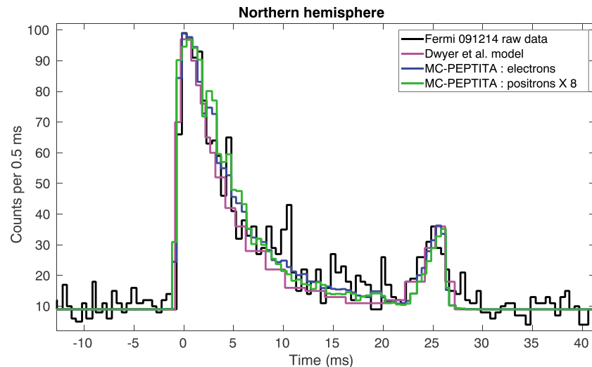
Figure 1. Time histogram of the Fermi 091214 event. Comparison between the data from Fermi GBM and the simulations of Dwyer et al. (both extracted from Briggs et al. [2011]) and our MC-PFEPTITA simulations (for electrons and positron). The counts for the positron histogram are multiplied by 8.
