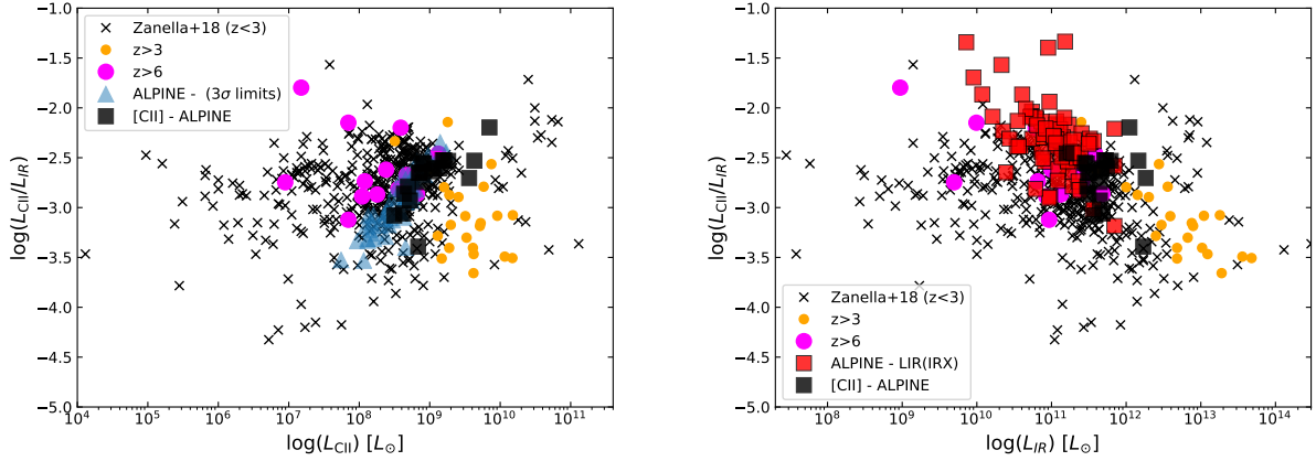
Fig. 8. L([\text{CII}])/L_{\text{IR}} versus L([\text{CII}]) (left panel) and L_{\text{IR}} (right) for the ALPINE sources and comparison samples where the [C II] line is detected. For the z > 6 sources, taken from the Matthee et al. (2019) sample, we adopt T_d = 45 K for the detections and L_{\text{IR}} upper limits. For galaxies not detected in the dust-continuum, we show their L([\text{CII}])/L_{\text{IR}} 3\sigma lower limit in the left panel as triangles. Right panel: L_{\text{IR}} limits of the ALPINE sources have been replaced by the L_{\text{IR}} values computed from the IRX– \beta relation, where possible.
