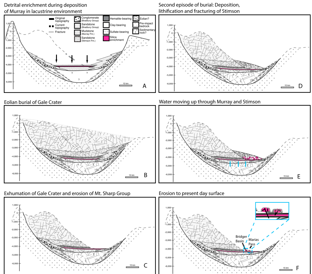
Figure 5. Proposed sequence of events: Hypothesized chronological sequence explaining the observed colocated detrital and diagenetic silica enrichment. The degree of aeolian burial is shown only to serve as illustrations. The dashed black line represents the approximate modern day geomorphology of Gale.
