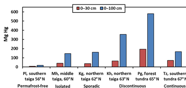
Figure 6. Total depth-integrated pools of Hg mass (Mg) in the upper 0–30 and 0–100 cm (red and blue columns, respectively) of WSL frozen peatlands in each permafrost zone. The stocks are calculated assuming the areal proportion of bogs from the landscape inventory across the WSL (Sheng et al., 2004).
