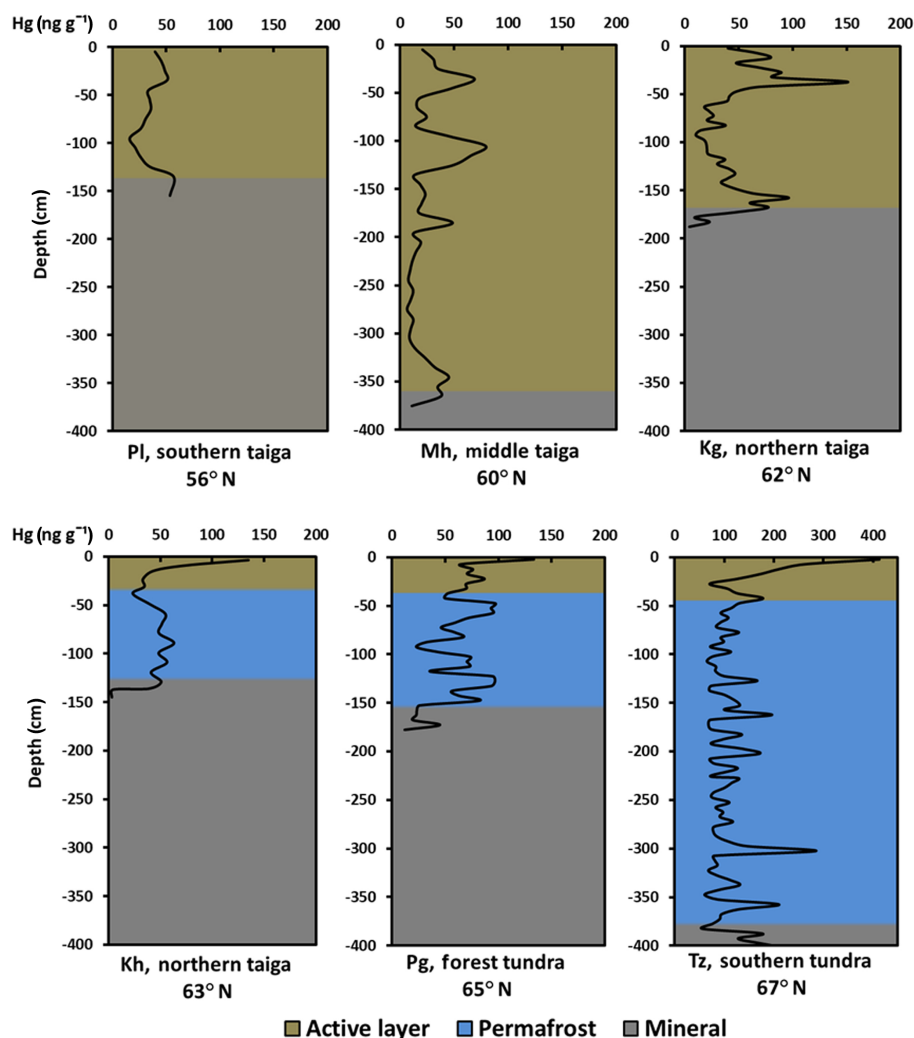
Figure 2. Vertical-depth profile distribution of total Hg (THg) in six peat cores across a 1700 km latitudinal transect of the WSL. Site location and physiogeographical parameters are shown in Fig. 1 and Table S1.
