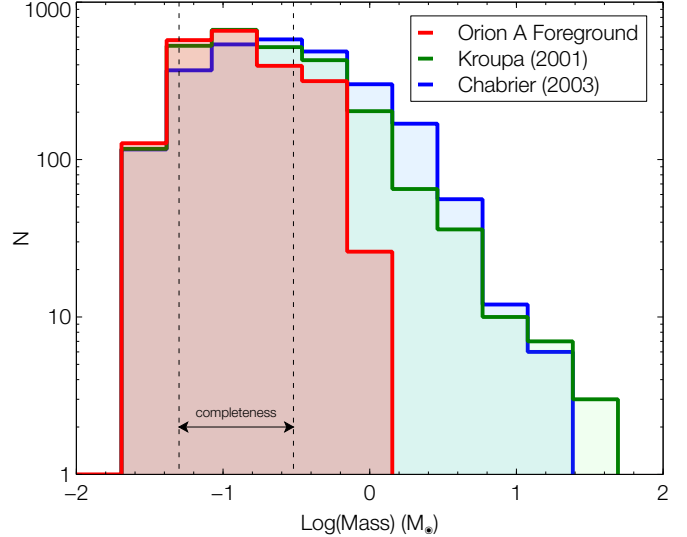
Fig. 10. Mass function of OriA-foreground over the completeness domain computed for 5 Myr and 10 Myr. The predictions of Chabrier (2003) and Kroupa (2001) mass functions are overplotted.
