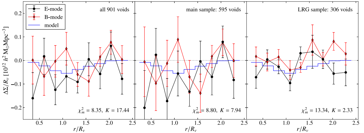
Figure 2. Void lensing signal in the range of r/R_v = 0.25, \dots, 2.4 of all voids ( left ), the main void sample ( centre ), and the LRG sample ( right ). The error bars show 68 per cent confidence intervals, estimated from 5000 bootstrap realizations of the mean in each bin. The blue curve shows the reference LW12 void model calculated from equation (3), binned in the same way as the data.
