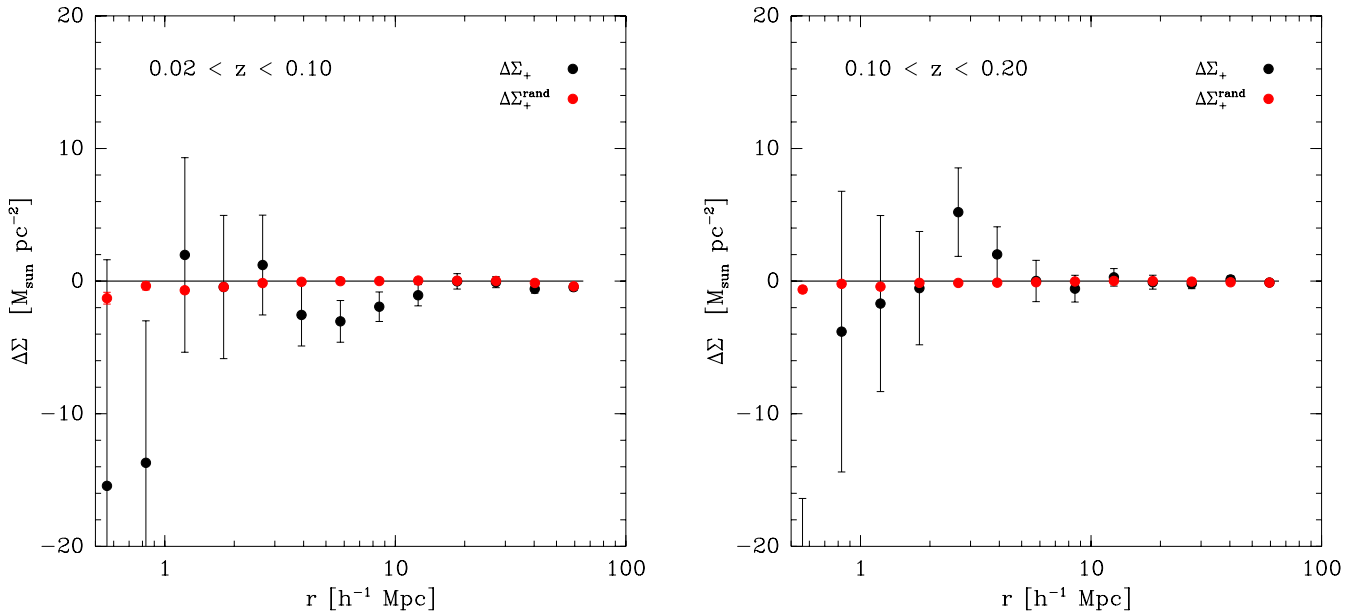
Figure A2. Lensing signal around voids ( black ) to the signal around random points ( red ) for two different redshift ranges. The signal was averaged as a function of physical radius rather than in units the void radius.
