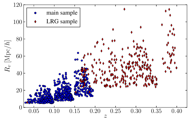
Figure 1. Redshift and size distribution of the voids used in this study. For each void, the redshift is taken to be the void centre’s and the radius is the one of a sphere with the same volume as the void.
