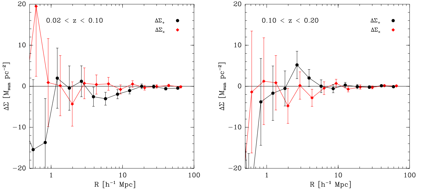
Figure A1. Lensing E mode ( \Delta\Sigma_+ , black ) and B mode ( \Delta\Sigma_\times , red ) for voids in two separate redshift bins. The signal was averaged as a function of physical radius rather than in units the void radius.
