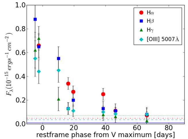
Figure 5. Flux evolution of the narrow Balmer and [O III] 5007 \text{ \AA} lines. The reported flux is the true flux of the lines above the continuum. The lines mark the values of the upper limits derived for the four emission lines in the host spectrum taken on 2013 November–December (see Table 4; dash-dotted, red, line refers to H\alpha emission; solid, blue, line to H\beta ; dotted, green, line to H\gamma ; and dashed, cyan, line to [O III] 5007 \text{ \AA} ). The last deep spectra of the host galaxy show that the contamination of the narrow line emissions from the host is negligible.
