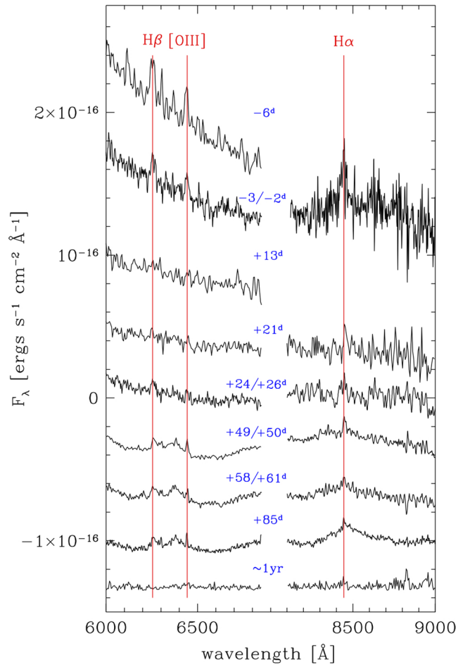
Figure 4. Spectral evolution of CSS121015 zoomed on the narrow H\beta , [O III] 5007 \text{ \AA} and H\alpha transitions. Wavelength and phases are as in Fig. 3.
