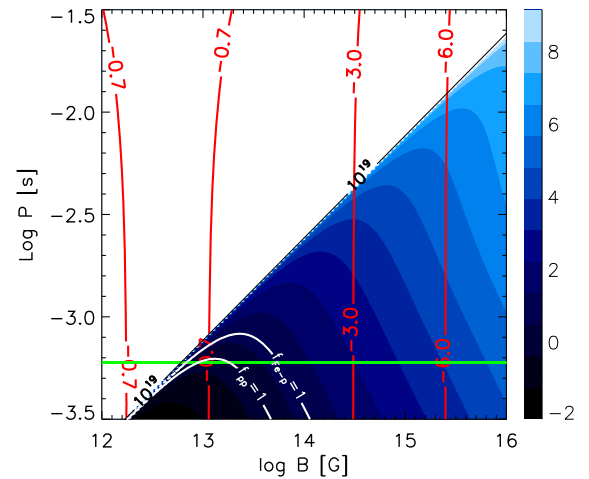
FIG. 1 (color online). Effective optical depth f_{pp} of hadron interactions in a 10M_{\odot} supernova ejecta at the time a pulsar with initial period P and surface magnetic field B accelerates 10^{19} \text{ eV} protons (regardless of energy losses). Pulsars that are capable of accelerating protons to above 10^{19} \text{ eV} lie under the black line ( \eta = 0.1 assumed). The blue shaded contours span from f_{pp} = 10^{-2} to 10^9 (among which f_{pp} = 1 is indicated in white). f_{\text{Fe-p}} = 1 is also shown for comparison. The overplotted red lines indicate the probability distribution function f(P, B) = f(P)f(B) of the pulsars. We assume that all pulsars have initial spin periods above the green line, which indicates the minimum spin period of a stable neutron star P_{\text{min}} \approx 0.6 \text{ ms} [17]. Both f_{pp} and f(P, B) are in logarithmic scale.
