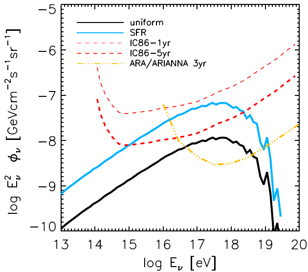
FIG. 3 (color online). The diffuse neutrino flux ( \nu_{\mu} + \nu_e + \nu_{\tau} after neutrino mixing in space) from an extragalactic newborn pulsar population that would produce the measured UHECRs. The source emissivity follows the SFR (blue) or is uniform over time (black). Overlaid are all flavor neutrino flux sensitivities of the IceCube detector after 1 year (red thin dash) and 5 years (red thick dash) of operations [28], and the expected 3-year ARA-37 sensitivities (orange dash dotted) [29].
