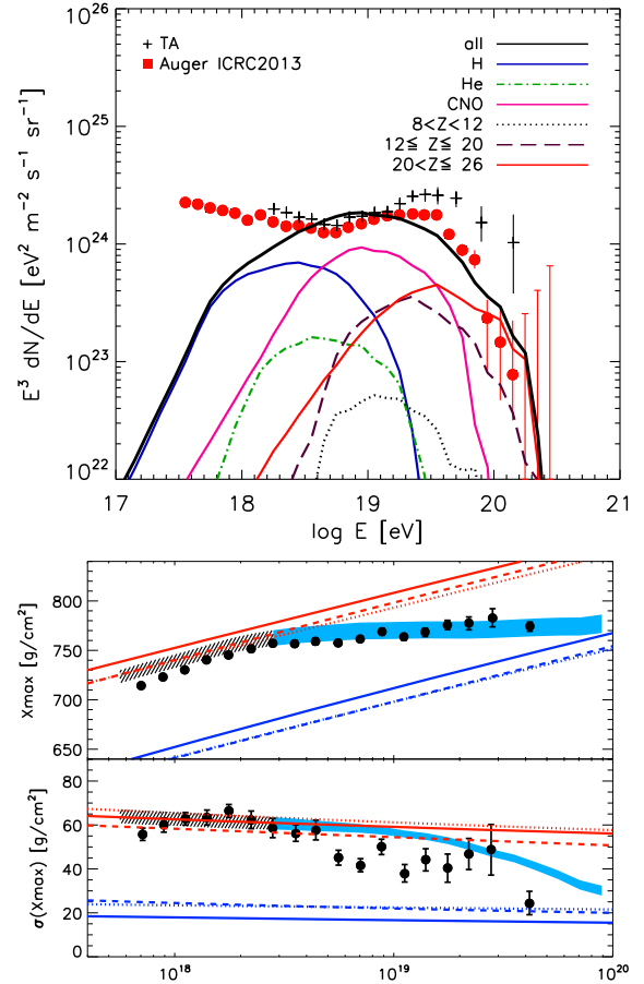
FIG. 2 (color online). Top: Spectrum of UHECRs from newborn pulsars, assuming source emissivity following SFR and injection composition: 50% H, 30% CNO and 20% Fe. Overlaid are measurements by the Auger Observatory [24] and the Telescope Array [25] with the energy rescaling suggested in Ref. [26]. Bottom: Values of estimations of UHECR composition, \langle X_{\max} \rangle and \text{RMS}(X_{\max}) of the Auger data [24] (black crosses) and simulation results with pulsar sources (blue shaded region where pulsars contribute to more than 80% of the total flux, hashed region for less). Three hadronic interaction models, EPOS-LHC (solid), QGSJetII-04 (dotted) and Sibyll2.1 (dash) are used to estimate the range of \langle X_{\max} \rangle and \text{RMS}(X_{\max}) [27]. The red and dark blue lines correspond to 100% P and 100% Fe.
