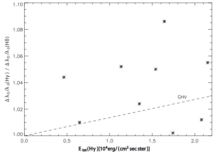
Fig. 5. Ratio of observed reduced Doppler widths \Delta\lambda_{\text{D}}/\lambda_0 of H \gamma and H \delta versus the total emission (“line radiance”) of H \gamma . The error bars are smaller than the symbols. Dashes give a mean of the three models with T_{\text{kin}} = 4300, 6000 and 8000 \text{ K} (all V_{\text{nth}} = 5 \text{ km s}^{-1} ) by Gouttebroze et al. (1993).
