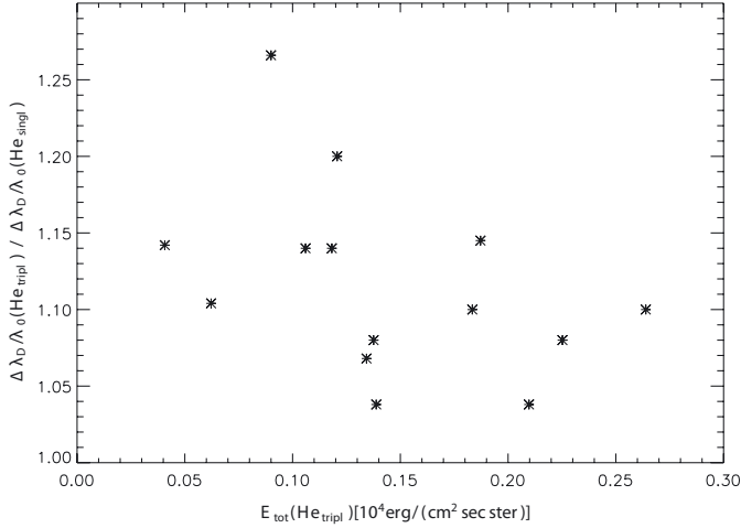
Fig. 6. Ratio of observed reduced Doppler widths \Delta\lambda_D/\lambda_0 of He I 4472 (triplet) and He I 5015 (singlet) versus the total emission (“line radiance”) of He I (triplet). The 1% accuracy (cf. Sect. 2.3) yields error bars of both, the ratio and the triplet radiance values slightly larger than the figure symbols.
