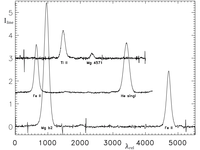
Fig. 2. Spectral line radiance, I_{\text{line}} [erg/(s cm 2 ster mÅ)], of Fe II 5168 with Mg b 2 5172 (lower), He 5015 (singl.) with Fe II 5018 (middle), ordinate shifted by +1.5 erg/(s cm 2 ster mÅ); and Mg 4571 with Ti II 4572 Å (upper curve), shifted by +3.0 erg/(s cm 2 ster mÅ), observed in prominence-15 (cf. Table 1). The abscissa gives relative wavelengths [mÅ].
