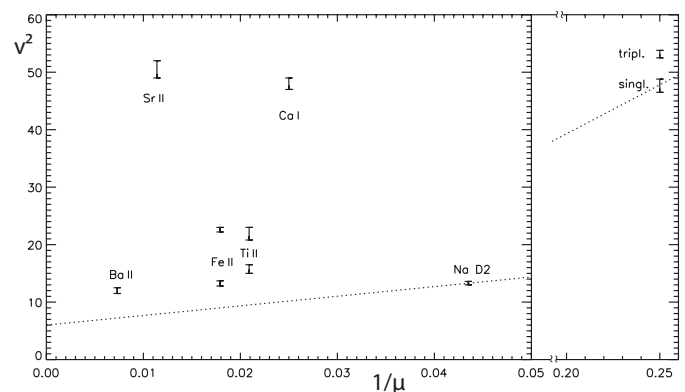
Fig. 1. Observed line widths V^2 = (c \cdot \Delta\lambda_D/\lambda_0)^2 [(km s -1 ) 2 ] versus inverse atomic mass 0 \leq 1/\mu \leq 0.05 of metallic lines and 0.20 \leq 1/\mu \leq 0.26 for helium singl. and tripl. (from Ramelli et al. 2012; listed in their Table 3, here with error bars). The dotted line connects Na D 2 and He singlet with apparent T_{\text{kin}} = 9950 K and V_{\text{nth}} = 2.5 km s -1 but does not fit any width of the other emission lines. The range 0.05 \leq 1/\mu \leq 0.20 is omitted.
