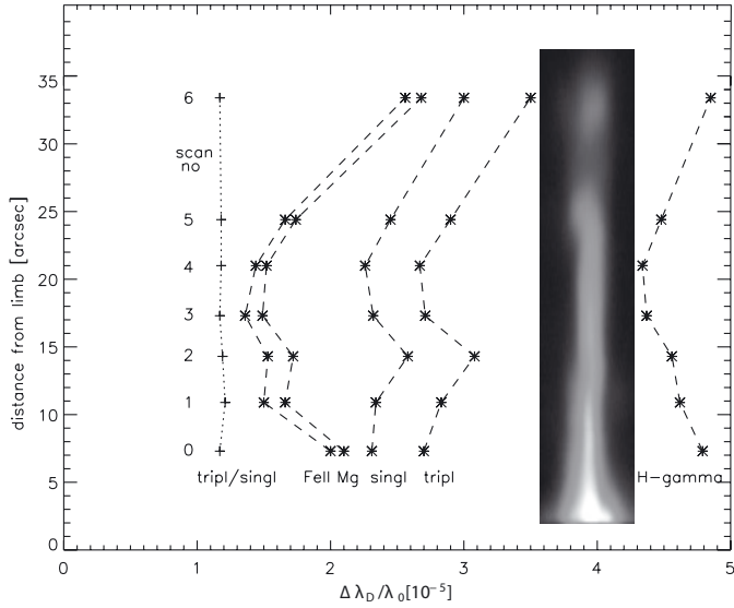
Fig. 7. Spatial variation (i.e. along the slit) of reduced Doppler widths \Delta\lambda_D/\lambda_0 of H\gamma , He I 4472 (triplet), He I 5015 (singlet), Mg b 2 5172, and Fe II 5018; also shown the (nearly constant) width ratio of He (tripl) and He (singl). The prominence No. 1 by chance extends along the direction of refraction, which necessarily is the slit orientation, cf. Sect. 2.1. Inserted is the Mg b 2 emission spectrum; \Delta\lambda = 0.8 \text{ \AA} .
