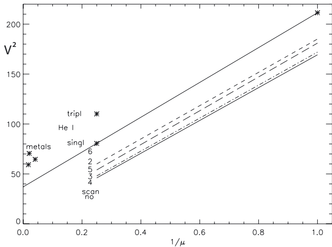
Fig. 8. Spatial variation of V^2 = (c \cdot \Delta\lambda_D/\lambda_0)^2 versus inverse atomic mass 1/\mu for 5 spatially distinct scans in prominence No. 1. Asterisks give scan-6 (in Fig. 7); the full line connecting H\gamma and He I 5015 (singlet), triplet and metals lay above that line (as in Fig. 1). The other lines similarly connect H\gamma and He I 5015 (singlet) values observed for scans-2 through -5 (in Fig. 7), and are of nearly the same steepness, T_{\text{kin}} = 10\,650 \text{ K} ; their ordinate off-sets correspond to 2 \leq V_{\text{nth}} \leq 6 \text{ km s}^{-1} .
