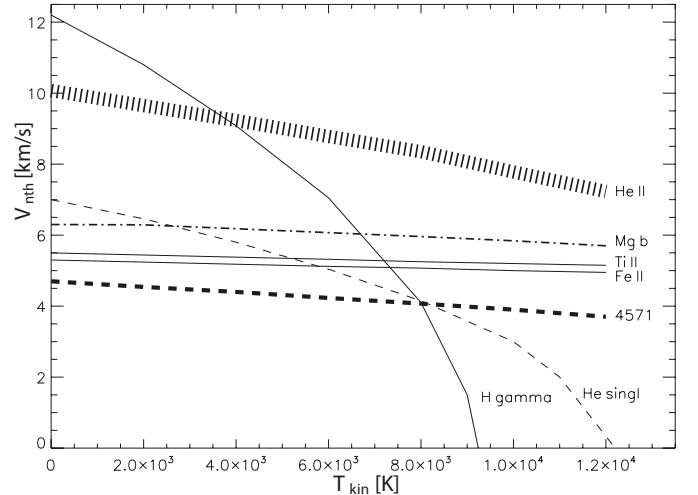
Fig. 4. Relation of V_{\text{nth}} and T_{\text{kin}} for each reduced line width, \Delta\lambda_{\text{D}}^{\text{obs}}/\lambda_0 , observed in prominence-15. The thickness of each curve represents the error bar of each observed \Delta\lambda_{\text{D}}/\lambda_0 .
