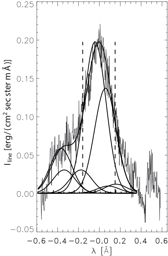
Fig. 3. He II 4686 Å emission, observed in prominence-15. It is fitted by a profile composed of the seven fine-structure components (cf. Ramelli et al. 2012) each with FWHM_{\text{int}} = 260 \text{ mÅ} , yielding a superposed profile with FWHM_{\text{tot}} = 320 \text{ mÅ} as observed.
