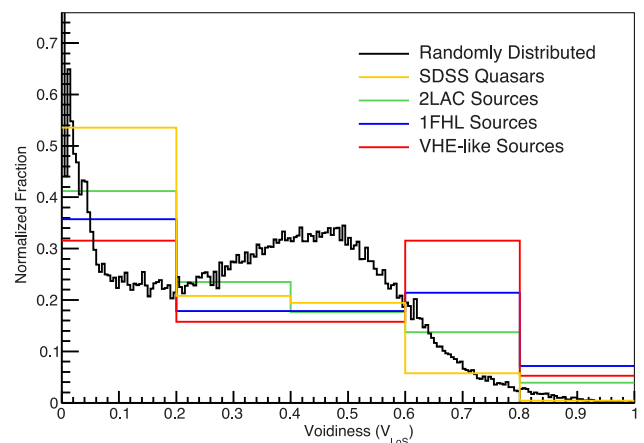
Figure 1. Normalized histograms of ‘voidiness’ V_{\text{LoS}} (equation 3) for the catalogue populations (randomly generated: black; SDSS: yellow; 2LAC: green; 1FHL: blue; VHE-like: red). See Table 2 for KS test results.
