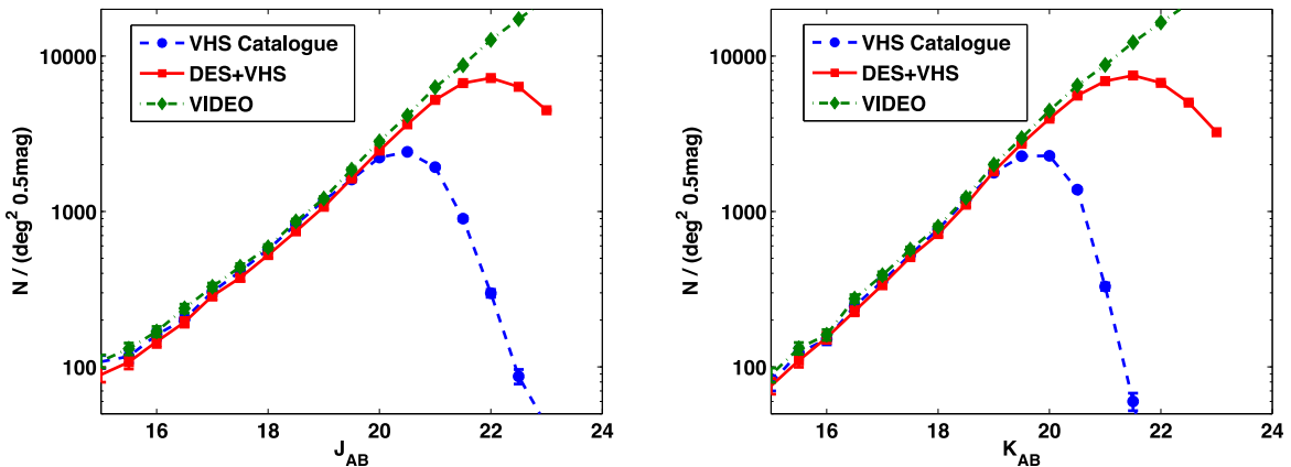
Figure 6. VHS J- and K_s -band number counts produced by running dual photometry on the VHS co-added images using the DES detection images (DES+VHS) compared to both VHS catalogue counts over the same area as well as deeper data from the VIDEO survey. All three distributions show good agreement at the bright end. The number counts are dominated by the extended sources and from this plot, the 80 per cent completeness for the VHS catalogues is J = 19.9 and K = 19.3 (appropriate for galaxies). The corresponding numbers for the DES+VHS dual photometry catalogue presented in this paper are J = 21.2 and K = 20.9 .
