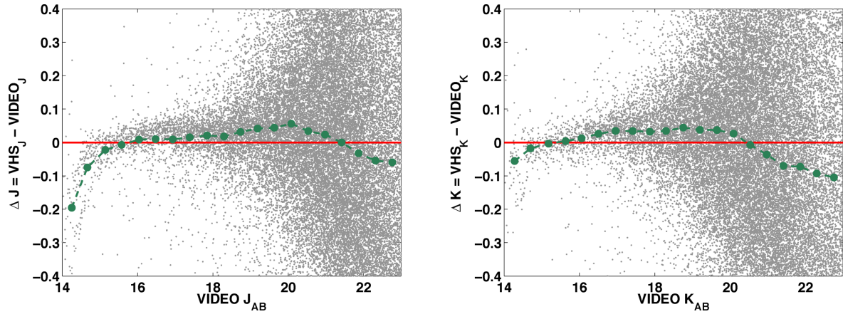
Figure 5. Difference between the SE extractor VHS forced photometry magnitudes and deeper VISTA VIDEO catalogue magnitudes in the J and K_s bands as a function of the VIDEO NIR magnitude. The dashed line corresponds to the median trend whereas the solid line marks an offset of 0 mag. The median offsets are +0.04 mag in J and +0.03 mag in K_s relative to VIDEO at the bright end, where the logarithmic magnitude distributions are expected to be roughly Gaussian.
