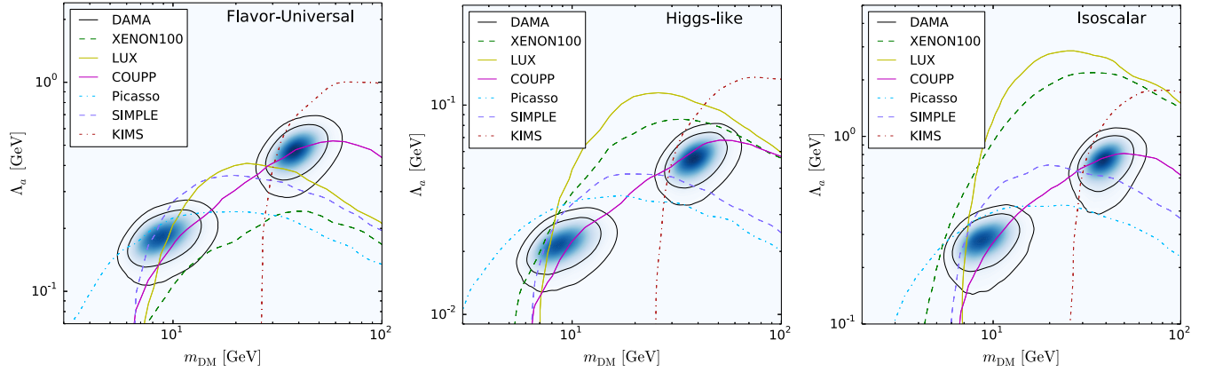
FIG. 1 (color online). Two-dimensional credible regions for DAMA (shaded area and black solid lines, 90% and 99% C.L.) and exclusion limits (99.5% C.L.) in the (m_{\text{DM}}, \Lambda_a) plane, for flavor-universal (left), Higgs-like (center), and isoscalar (right) couplings.
