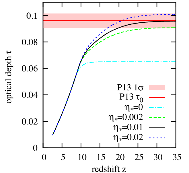
Figure 3. Optical depth as a function of redshift for different choices of the SFE \eta_* and comparison to the observational constraint by the Planck Collaboration XVI (2014). The contribution from Pop I/II star formation yields a baseline value of \tau_{\text{Pop I/II}} = 0.065 , and the complete model results in values in accordance with the observational constraint for the three selected SFEs.
