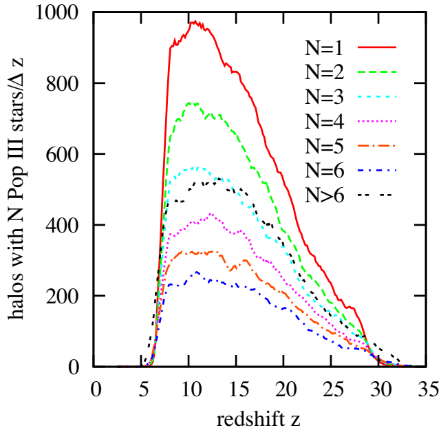
Figure 9. Number of Pop III stars per minihalo for our standard model. At any redshift, this plot illustrates how many new haloes form with N Pop III stars per unit redshift bin. Although we use a simple probabilistic IMF sampling, this approach reproduces the results of numerical simulations that most of the primordial stars form in higher multiple systems.
