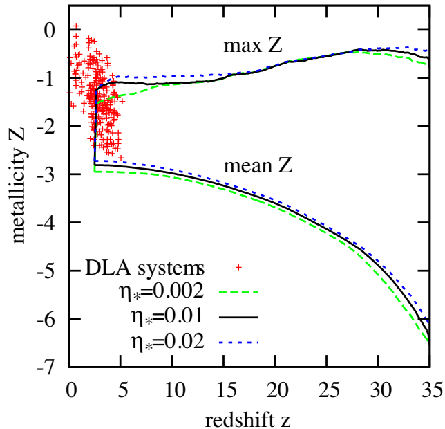
Figure 4. Mean and maximal metallicities in the proto-Milky Way-like halo, as a function of redshift, for different SFEs. The model predictions are compared to observed DLA metallicities (Rafelski et al. 2012). Evidently, we can conclude that there were already sufficiently enriched regions at high redshifts to explain the DLA metallicities, which in turn supports our metal enrichment model.
