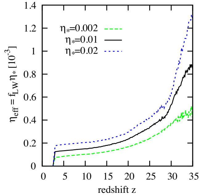
Figure 7. Overall Pop III SFE as a function of redshift. The parameter \eta_{\text{eff}} combines the two individual efficiencies in equation (20), and indicates which fraction of the total baryonic mass in the halo, on average, turns into Pop III stars.
