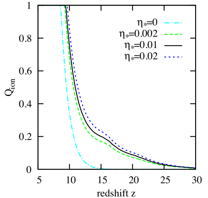
Figure 14. Volume filling fraction of the ionized IGM as a function of redshift. Values for the standard case ( f_{\text{esc, III}} = 0.7 and f_{\text{esc}} = 0.3 ), whereas \eta_* = 0 represents the Pop I/II-only model for comparison. In all models, reionization occurs between z = 8 and 10.
