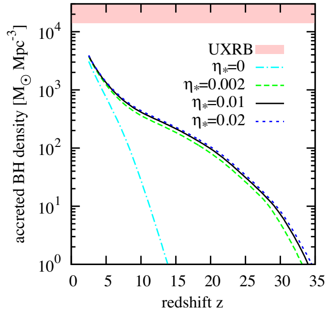
Figure 5. Mass density accreted on to BHs as a function of redshift and upper limit based on the observationally inferred UXR. It is evident that our model does not violate this empirical constraint.
