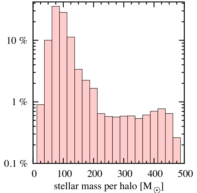
Figure 10. Distribution of the stellar mass per halo. Most of the haloes have a stellar mass content of \sim 100 M_{\odot} and the broad distribution from \sim 25 to \sim 500 M_{\odot} reflects the stochastic nature of Pop III star formation and disc fragmentation.
