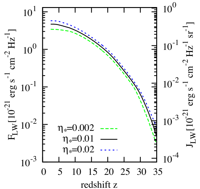
Figure 8. Average background flux of LW photons as a function of redshift. Our model prediction is consistent with the results by Johnson, Greif & Bromm (2008).
