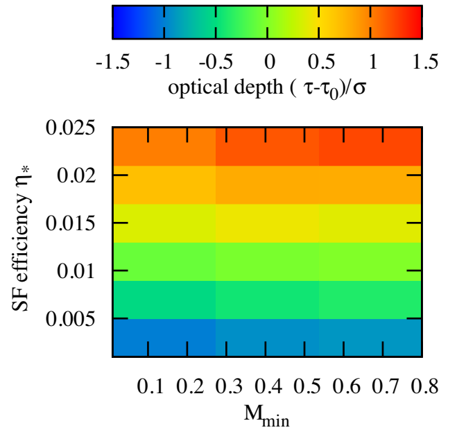
Figure 2. Optical depth minus the Planck Collaboration XVI (2014) value normalized to the 1\sigma error as a function of the SFE and of the lower IMF mass limit. Since ionizing photons are mainly produced by high-mass stars, the lower IMF mass limit hardly affects the optical depth. However, the optical depth crucially depends on the SFE and is therefore used to calibrate this key model parameter.
