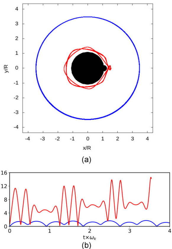
Figure 4. (a) Trajectory in the rotating frame and (b) temporal evolution of the eccentricity. The innermost particle (red line) is at 1.74 R and the outermost one (blue line) at 3.48 R , and both are initially in circular orbits. The parameters of the central body are \lambda = 0.471 and \mu = 5 \times 10^{-3} .
