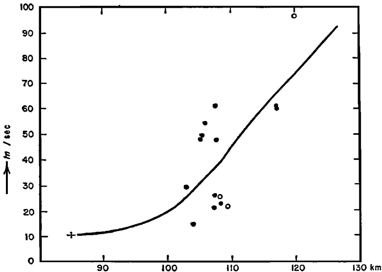
Fig. 4. Wind velocities in the 100-km region, derived from measurements of the trail of March 10, 1959, kindly communicated by Miss Baguette. Open circles represent uncertain values. The plot at 85 km is derived from meteor measurements [Greenhow, 1959].
