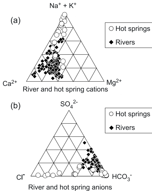
Figure 2. (a) Cation and (b) anion triangular diagrams showing river (filled diamonds) and hot spring (open circles) chemistry. Rivers are dominated by carbonate dissolution, with high Ca 2+ and Mg 2+ , while hot springs show a strong silicate alteration influence with Na + and K + making up most of the cation budget. Both river and hot spring anion balances are controlled by bicarbonate with some hot springs showing variable but strong Cl - enrichment.
