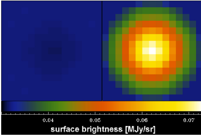
Fig. 2. Scattered light images of a model core with overall properties like L1506C using an MRN size distributions extending to grain sizes of 0.25 \mu\text{m} (left) and 0.65 \mu\text{m} (right). The total dust mass is kept constant. The background surface brightness is 0.032 \text{ MJy/sr} and the coreshine surface brightness above background is 0.04 \text{ MJy/sr} for L1506C.
