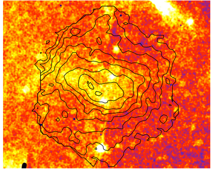
Fig. 1. Core L1506C seen in coreshine and thermal dust emission. Image: Spitzer IRAC channel 1 map of L1506C. North is up and east is to the left. Non-saturated point sources have been identified and masked using sExtractor . Contours: MAMBO 1.2 mm observations (Pea10), in steps of 0.5 mJy/beam up to 5.5 mJy/beam. The field of view is 20' \times 13' .
