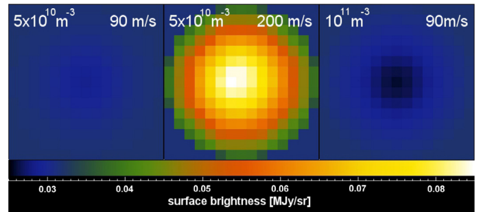
Fig. 6. Scattered light images of a model core like L1506C assuming a growth time of 10^6 yr. In each image, the peak core density is given left, the right number is the turbulent speed in the largest eddy.
