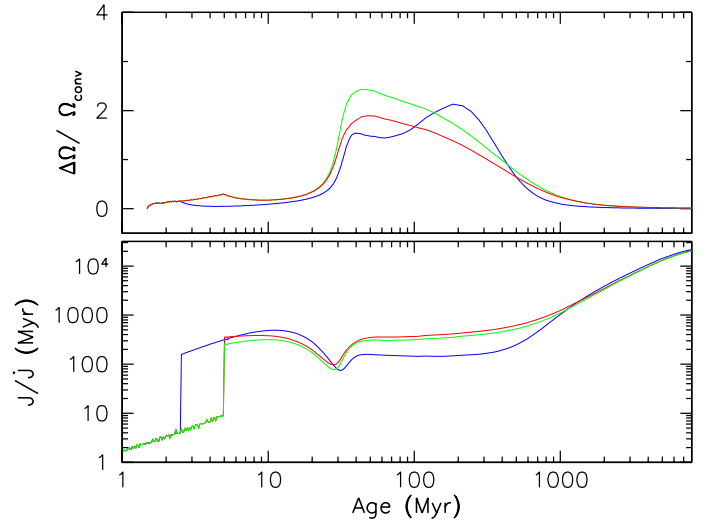
Fig. 5. Upper panel: velocity shear at the base of the convective zone (\Omega_{\text{core}} - \Omega_{\text{env}})/\Omega_{\text{env}} in the case of fast (blue), median (green), and slow (red) rotator models. Lower panel: spin-down time-scale ( J/J ) expressed in Myr, in the case of fast (blue), median (green), and slow (red) rotator models.
