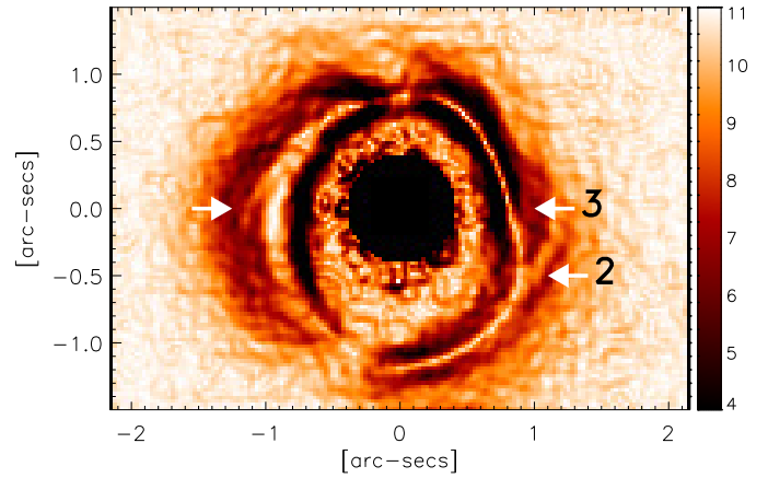
Fig. 6. P_1 images at H band after applying a Sobel filter to highlight the regions of the image with edges. The three arrows indicate spiral arms on the disk. For comparison, we used the same notation as in Casassus et al. (2012) (see also Rameau et al. 2012) to label the spiral arms. The spiral arm labeled “2” perfectly matches its equivalent in Casassus et al. (2012). The spiral arm labeled “3” is barely visible in our images. The spiral arm on the east side is detected for the first time. Color bar is in arbitrary units.
