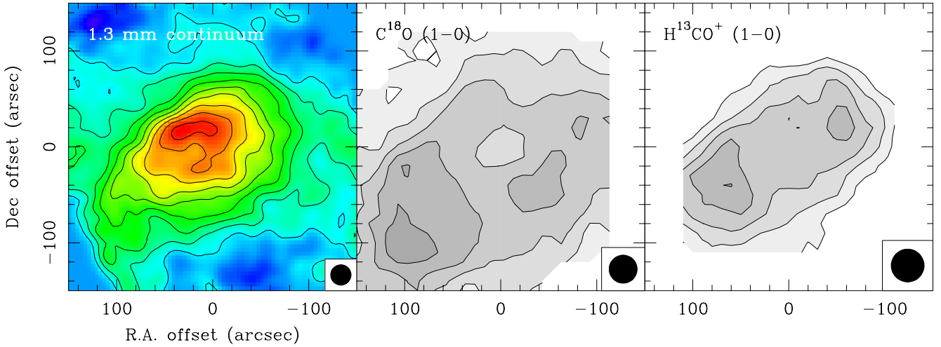
Fig. 1. Left panel: 1.3 mm continuum emission observed in L1498 (Tafalla et al. 2004). Contour levels start at 2 mJy per 11'' beam and increase by steps of 2 mJy per 11'' beam. Middle panel: C^{18}O(1-0) integrated intensity. Contour levels start at 0.2 K km s -1 ( 6.2\sigma ) and increase by steps of 0.2 K km s -1 . Right panel: H^{13}CO^+(1-0) integrated intensity. Levels start at 0.1 K km s -1 ( 5.9\sigma ) and increase by steps of 0.1 K km s -1 . In each panel the spatial resolution of the map is indicated by a filled circle.
