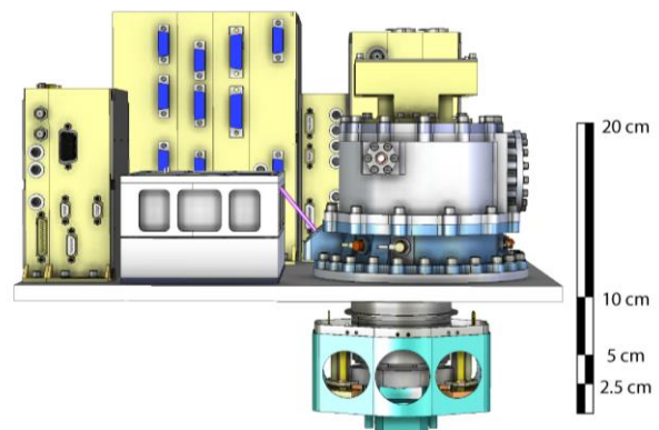
Figure 1. The lightweight and compact CRATER design enables versatile deployment options on an upcoming commercial lunar rover or lander concept.
