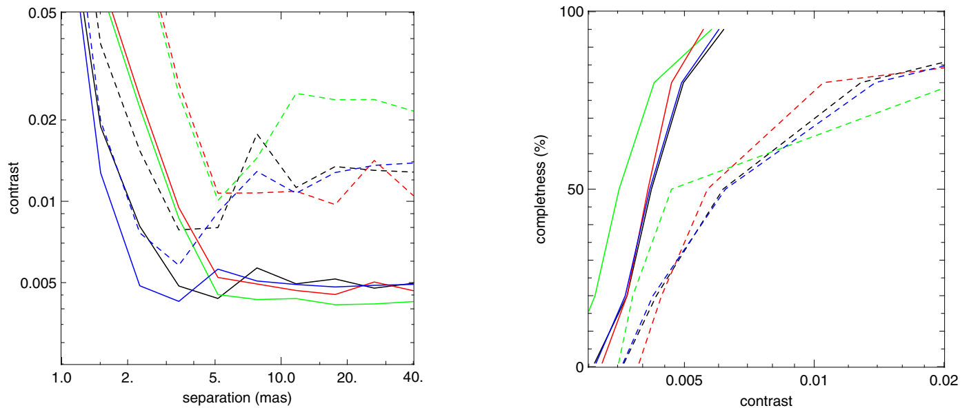
Fig. 5. Left: 3\text{-}\sigma sensitivity versus separation for a completeness level of 80%. Right: completeness in the separation range 6–40 mas versus contrast. Simulations are for a single snapshot pointing (dashed lines) and for five pointings separated by one hour (solid lines). Colours are for the four configurations displayed in Fig. 4. The black curves are for the U1-U2-U3-U4 configuration displayed in Fig. 1. The contrast axes can be scaled for any accuracy on the closure phase (here \sigma = 0.25 deg).
