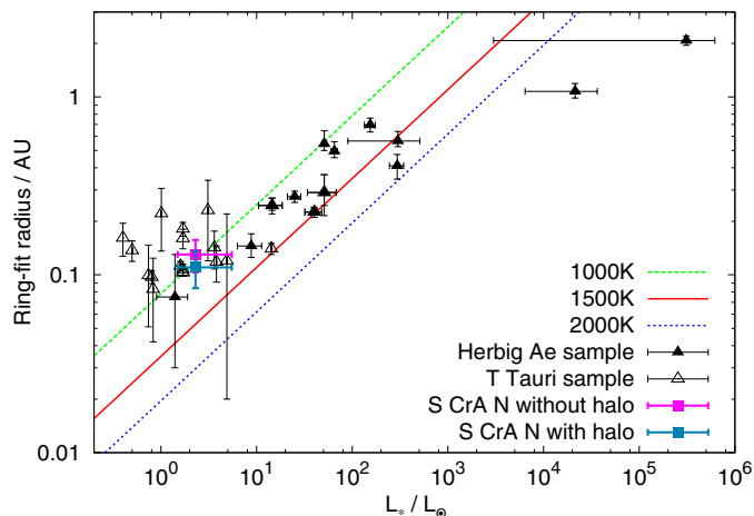
Fig. 5. Location of S CrA N in the size-luminosity diagram: K -band ring-fit radii derived with a geometric ring-star model (pink square, \approx 0.13 AU) and a ring-star-halo model (blue square, \approx 0.11 AU); see Tables 3 and 1 for the stellar parameters used. The lines indicate the predicted theoretical dependence of the K -band radius on the luminosity (Monnier & Millan-Gabet 2002). Predictions of models including backwarming are discussed in Sect. 4. The filled black squares are a sample of Herbig Ae stars (Monnier et al. 2005). The open black squares represent a sample of TTS (Pinte et al. 2008).
