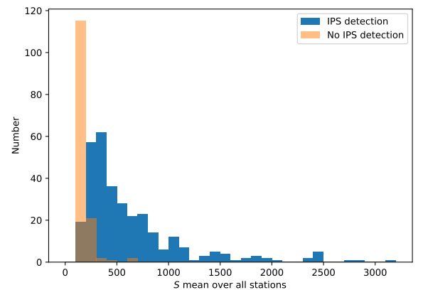
Fig. 14. Histogram of the mean LBCS statistic across all baselines for sources with and without IPS counterparts.
