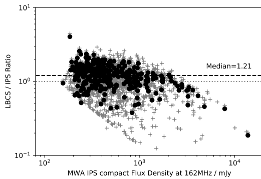
Fig. 16. Comparison of IPS flux densities compared with those inferred from LBCS via Eq. (2). Plus signs (+) are all LBCS sources with a counterpart; filled circles are those sources in the region 7\text{ h} < \text{RA} < 11\text{ h} , +6^\circ < \delta < +18 where both surveys have good data.
