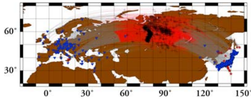
Figure 1. Event-receiver geometry, with great circle ray paths. The portions of the great circles which sample D'' are shown in red. Blue reversed triangles and red stars show the sites of stations used in our study and earthquakes studied, respectively. Plus signs are the bounce points indicated by geometrical optics.
