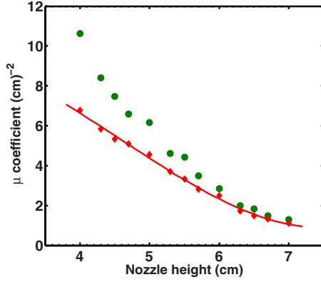
FIG. 8. (Color online) The nonlinear saturation coefficient \mu , as a function of the nozzle height H . The solid circles are the values deduced from fits to Eq. (4). Diamond symbols show the kinematic estimate \mu \approx (\omega_c/2U_c)^2 for each height, discussed in the text. The solid line is a cubic polynomial model of the kinematic estimates.
