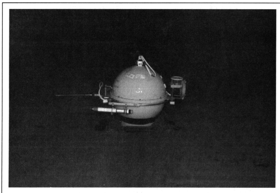
Fig. 2. The BBOBS on the seafloor at the FP6 station, which is 200 km south of the Macdonald hot spot at a depth of 4400 m. Original color image appears at the back of this volume.
