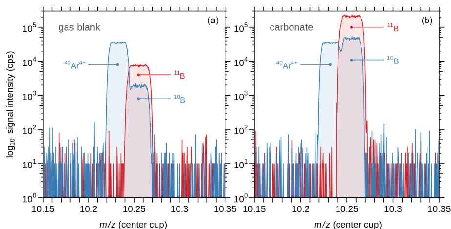
Figure 1. Mass scans over atomic masses 10 (blue) and 11 (red) using Daly detectors, where peak center coincidence appears at \sim 10.25 amu in the center cup. (a) Gas blank (laser off), showing the typical double peak of ^{40}\text{Ar}^{4+} and ^{10}\text{B} , and the ^{11}\text{B} peak. (b) Signal of ablated calcium carbonate (laser on). The baseline exhibits only electronic noise from the Daly detectors, but no sign of unresolved interferences on ^{10}\text{B} as matrix-induced scattered Ca ion. Note that the signal intensity is on a logarithmic scale.
