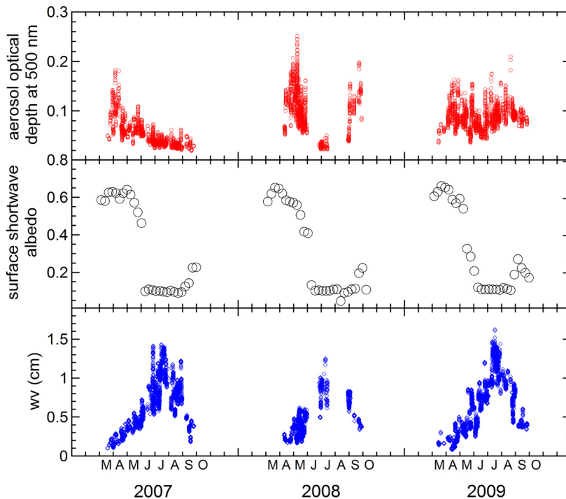
Figure 10. Top panel: aerosol optical depth at 500 nm. Bottom panel: column water vapour (wv) derived from Cimel observations. Center panel: MODIS derived 8-day surface shortwave albedo during the period March-October of the years 2007-2009.
