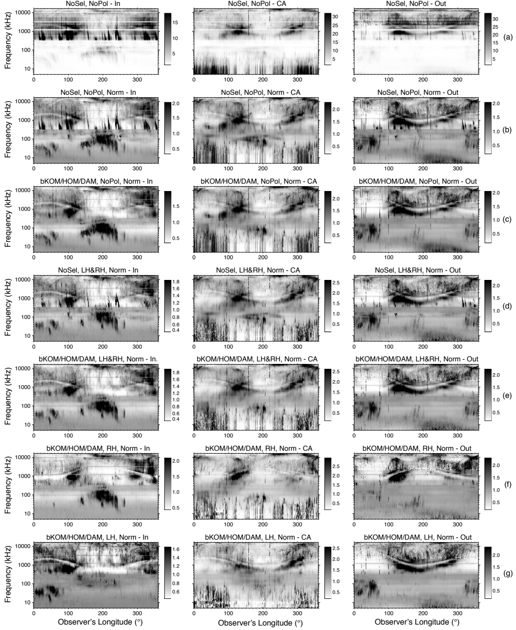
Figure B1. Overview of stacked frequency-longitude plots for various catalog and/or polarization selections. The frequencies cover the range 5-16125 kHz following a logarithmic scale, and longitude bins are 1^\circ wide. The 3 columns correspond to inbound [In], near-CA [CA] and outbound [Out] intervals. Row (a) [NoSel, NoPol] was obtained without any selection, just by stacking all data. The grey scale is linear, in multiples of 10^{-20.5} \text{ Wm}^{-2} \text{ Hz}^{-1} at 1 AU from Jupiter. Row (b) [NoSel, NoPol, Norm] corresponds to the same selection as row (a), with each line of the dynamic spectrum divided by its average value, equalizing the contrast at all frequencies. The grey scale, still linear, is now in relative units of average flux density at each frequency. This display is used for all subsequent rows. Row (c) [bKOM/HOM/DAM, NoPol, Norm] results from a selection of auroral components bKOM, HOM and DAM from our catalog. Row (d) [NoSel, LH&RH, Norm] is obtained from a selection in polarization only, using the intervals
