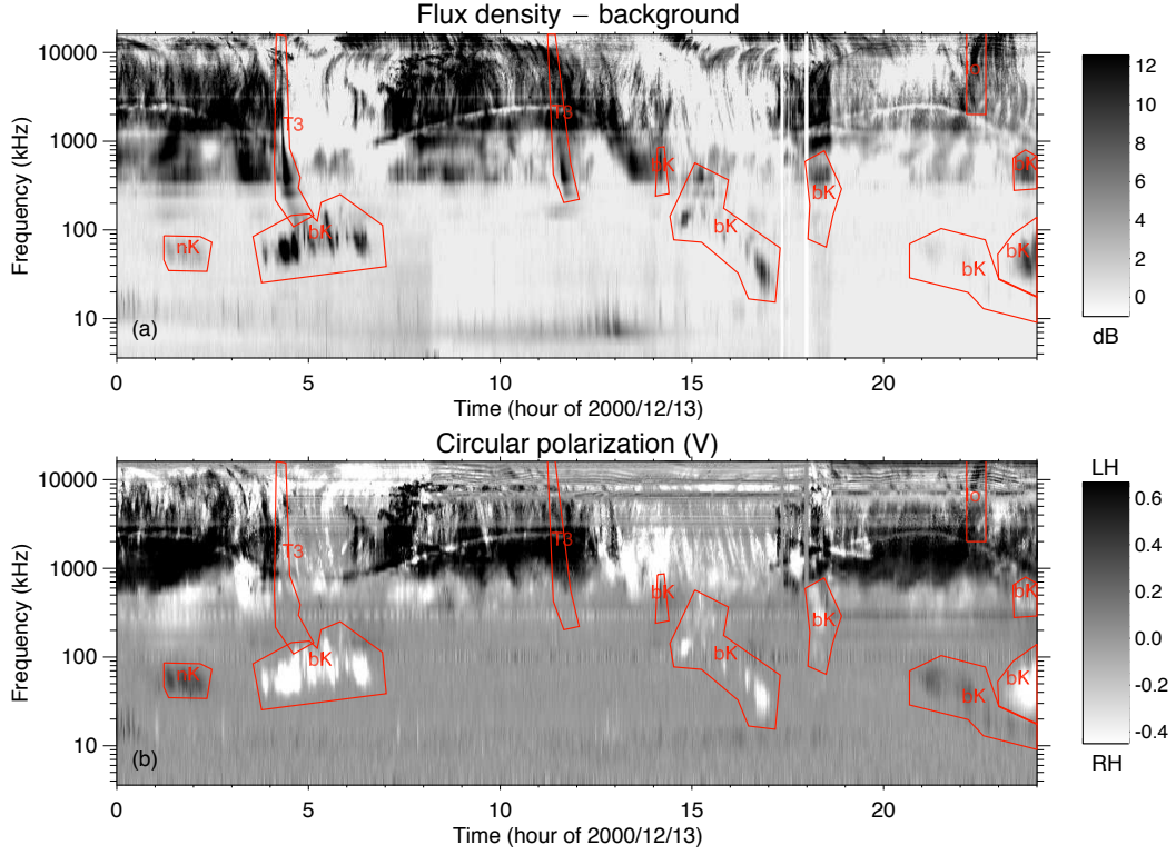
Figure 2. Example of 24-hour dynamic spectra (from 2000/12/13, i.e. day 348 of year 2000) used for building our radio components catalog, with indication of catalogued events (red contours). (a) Detrended flux density measured by RPWS, with background subtracted. The flux density scale is in dB above the background. (b) Circular polarization V . Radio components were visually identified according to their time-frequency morphology and polarization. Catalogued components include solar type III bursts ( T3 , unpolarized thus invisible in panel (b)), Jovian bKOM ( bK ), nKOM ( nK ), and Io-induced DAM ( Io ). Jovian radio components show a clear 10-hour periodicity linked to Jupiter's rotation. A curved, 10-hour modulated attenuation 'lane' is visible in the range 0.7–3 MHz.
