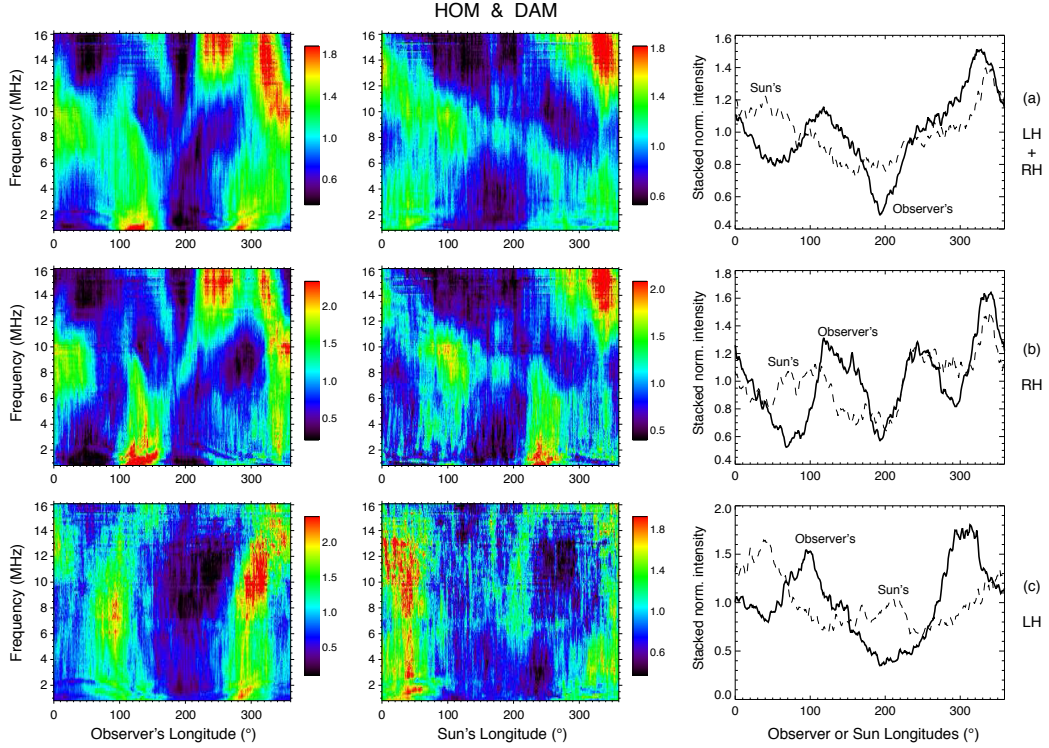
Figure 4. Stacking of RPWS measurements of HOM and DAM emission over the entire Cassini-Jupiter flyby in the range 0.8 – 16.1 MHz. In the first column, the dynamic spectrum is stacked as a function of Observer’s longitude (in 1^\circ wide bins). Each line of the dynamic spectrum has been divided by its average value, equalizing the contrast at all frequencies, as defined in Figure B1b. In the second column, stacking is similarly done, but as a function of the Sun’s longitude. On the average, each pixel of these dynamic spectra corresponds to the stacking of \geq 430 RPWS measurements. The contrast of the display is slightly stretched relative to Figure 3, for enhancing the various components. In the third column, the two curves in each panel result from the integration over all frequencies of the two dynamic spectra on the same line, and show intensity profiles versus longitude (Observer’s = solid line, Sun’s = dashed line). These profiles have been smoothed over 3 consecutive pixels in order to reduce the influence of small spikes. Row (a) corresponds to RH + LH polarized emissions ( 0.02 \leq |V| \leq 1.05 ), row (b) to RH emissions only ( -1.05 \leq V \leq -0.02 ) and row (c) to LH emissions only ( 0.02 \leq V \leq 1.05 ).
