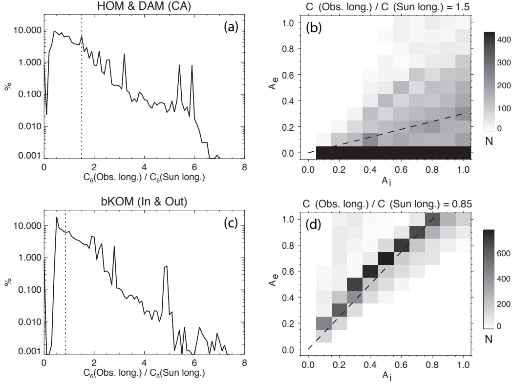
Figure 7. Summary results of the parametric study described in the text for modelling the superimposed internal and external controls of Jovian auroral radio components. (a) Distribution of the computed ratio C_6(\text{Observer's longitude})/C_6(\text{Sun's longitude}) along the near-CA trajectory. (b) Distribution of the couples of amplitudes (A_i, A_e) from study (a) and equation (3) that lead to a ratio 1.50 \pm 0.05 (dotted line in (a)). The dashed line is the linear fit (with a constant set to 0) to the weighted average in each column. (c) Same as (a) but computed along inbound and outbound legs of Cassini's trajectory only. (d) Distribution of couples (A_i, A_e) from study (b) that lead to a ratio 0.85 \pm 0.05 (dotted line in (c)), and linear fit to the weighted average in each column.
