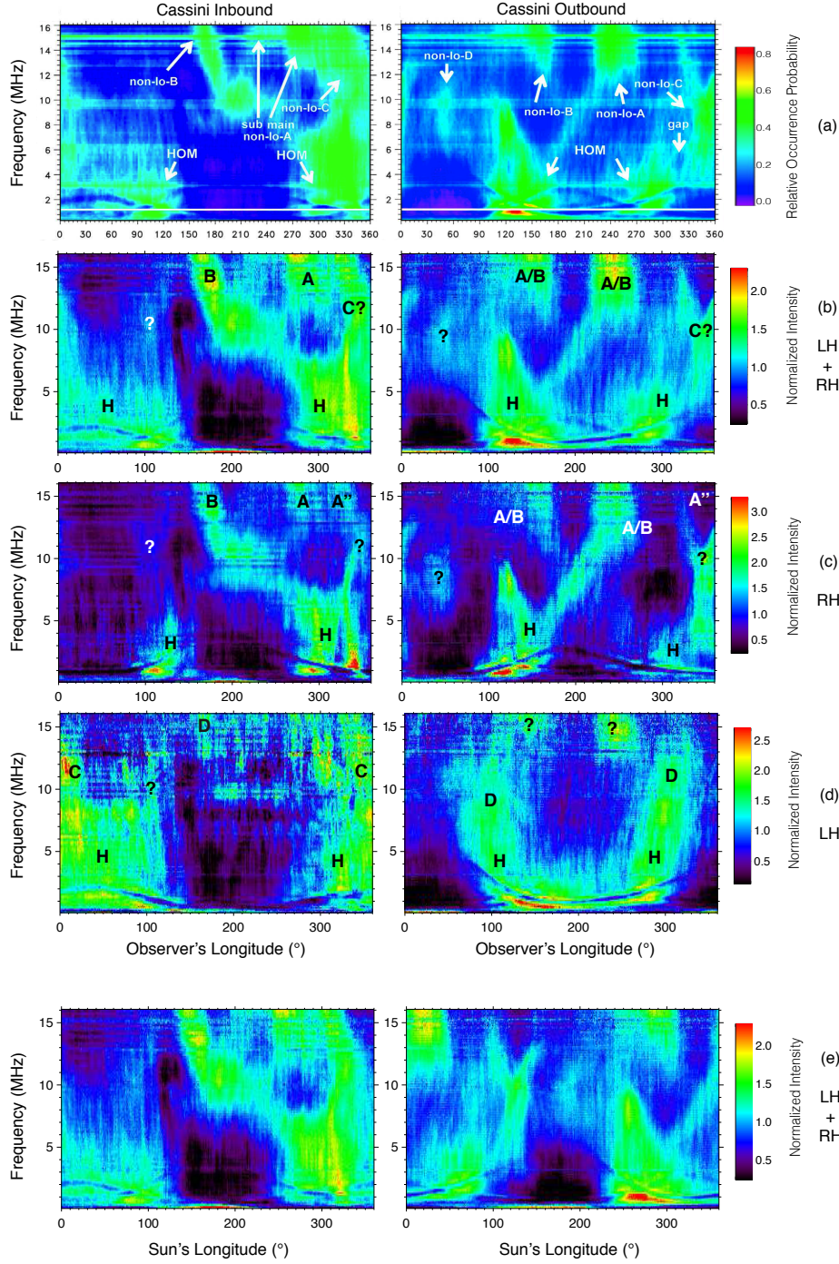
Figure 3. Inbound (first column) and outbound (second column) stacked dynamic spectra of auroral HOM and DAM versus frequency and Observer's (rows (a-d)) or Sun's longitude (row (e)), in 1^\circ longitude bins. Intensities in dB are stacked and then each row is divided by its average value. The linear frequency scale, emphasizes HOM and DAM while marginalizing bKOM at the bottom of the plots. Row (a) is reproduced from Fig. 4 of Imai et al. (2011), with identified radio components labelled in white. Following rows result from our reprocessing of RPWS data, with a selection in polarization ( -1.05 \leq V \leq 0.02 and/or 0.02 \leq V \leq 1.05 ) and from our catalog (bKOM, HOM and DAM). The color scale (in relative units of average flux density at each frequency) has been adjusted to match that of row (a). Our identifications of radio components are
