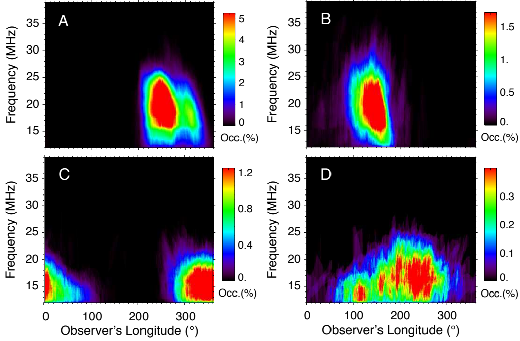
Figure 8. Occurrence probability of each auroral (satellite-independent) DAM component, from the Nançay Decameter Array catalog of Marques et al. (2017), as a function of Observer's longitude (in 1^\circ bins) and frequency (in 100 kHz bins). The number of occurrences of the corresponding emission in each bin is divided by the number of observations performed in the same bin. As seen from Earth, A & B originate from the Northern hemisphere, C & D from the South, B & D from the dawn side and A & C from the dusk side of the magnetosphere.
