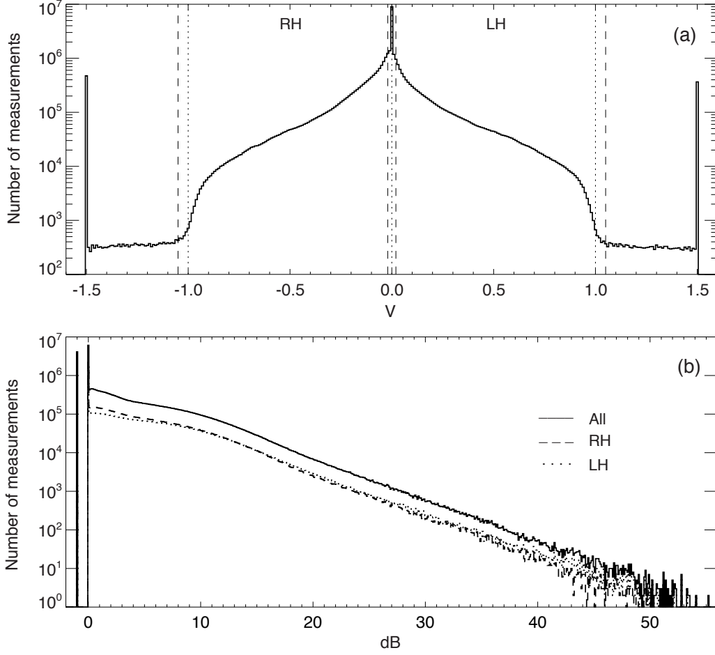
Figure A2. Distributions of circular polarization and calibrated intensities measured by Cassini-RPWS-HFR at Jupiter. (a) Histogram of circular polarization (V) values. The peak at V = 0 corresponds to unpolarized measurements (background, Solar type III bursts). Inversion results are arbitrarily limited to \pm 1.5 . Dotted lines indicate V=0, \pm 1 . Dashed lines delimit our defined ranges of RH ( -1.05 \leq V \leq -0.02 ) and LH ( +0.02 \leq V \leq +1.05 ) polarized emissions. (b) Histograms of measured flux densities, independent of V (All = solid line), RH polarized (dashed line), and LH polarized (dotted line).
