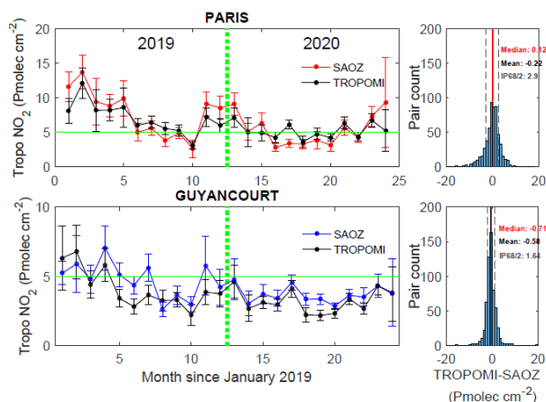
Figure 4: Left panels: Monthly mean tropospheric NO 2 and 2 \sigma standard error above Paris (upper panel) and Guyancourt (bottom panel) measured by ground-based SAOZ instrument (color lines) and TROPOMI satellite instrument (black lines). Right panels: Histogram of TROPOMI-SAOZ differences at Paris (upper panel) and Guyancourt (bottom panel). Vertical lines represent the median, mean and dispersion by the half of the 68% interpercentile (IP68/2).
